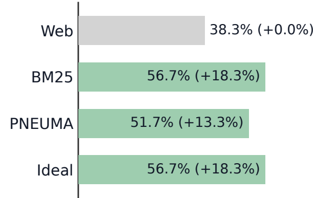
Semantic match
