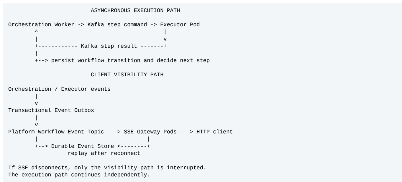
Figure 14 - Asynchronous execution and SSE visibility are separate paths
