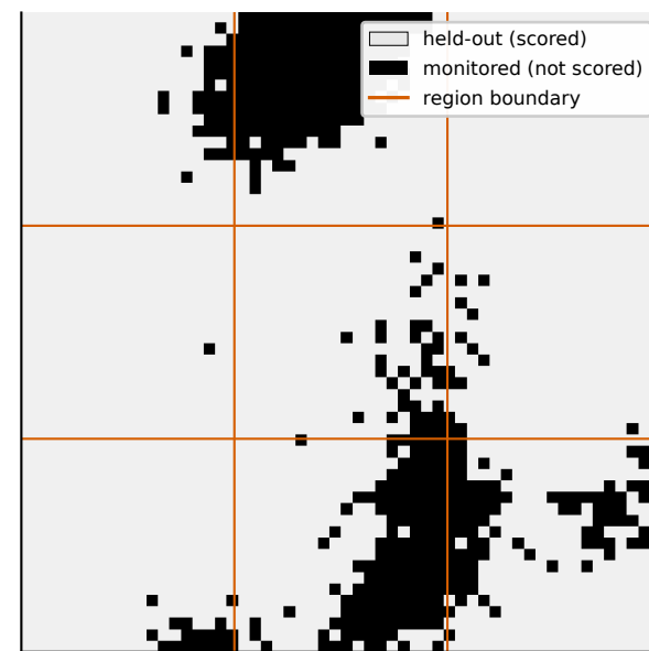
(c) evaluation cells for the design in (a)
