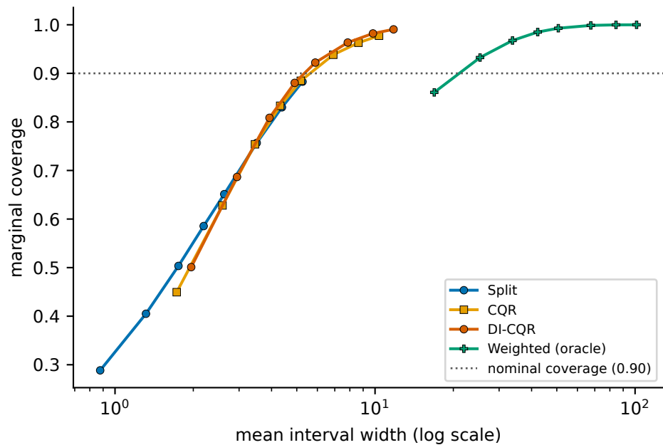
(a) moderate covariate-driven bias
