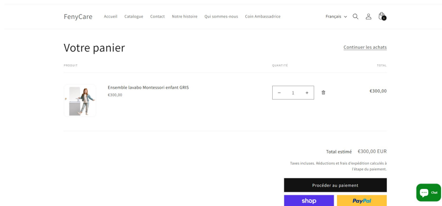
FIGURE 6.2 – Page panier
