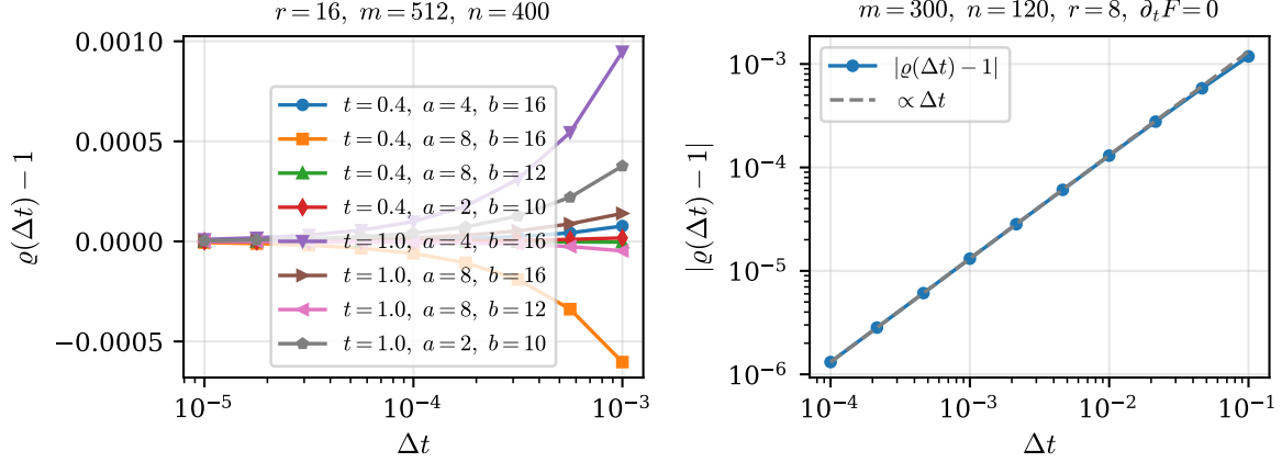
Figure 2: Verification of Theorem 5.4. Left: \varrho(\Delta t) - 1 for one step from rank-16 KL-gauge truncations of the Burgers reference at t = 0.4 and t = 1.0 and several (a, b) ; right: |\varrho(\Delta t) - 1| for constant dynamics on random matrices, with the reference slope \propto \Delta t .
