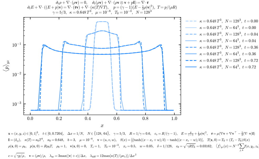
Figure 6: Pressurized-slab pressure profiles at the indicated times for grids with N = 64 and N = 128 cells per direction. The ordinate is the yz -averaged pressure \langle p \rangle_{yz} , and the abscissa is the coordinate x on the unit periodic domain. Solid and dashed curves distinguish the two resolutions. The conductivity is \kappa(T) = 0.648T^3 , the dynamic viscosity is \mu = 10^{-6} , and the ratio of specific heats is \gamma = 5/3 . This comparison assesses the spatial discretization of the deterministic flow calculation.
