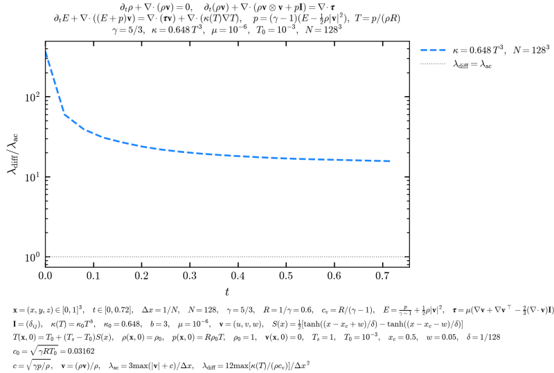
Figure 7: Diffusion-to-acoustic rate ratio \lambda_{diff}/\lambda_{ac} versus time t for the pressurized-slab calculation with N = 128 cells per direction. Here \lambda_{diff} = 12 \max[\kappa(T)/(\rho c_v)]/\Delta x^2 is the thermal-diffusion rate and \lambda_{ac} = 3 \max(|\mathbf{v}| + c)/\Delta x is the acoustic rate. The symbols \rho , c_v , \mathbf{v} , c , and \Delta x = 1/128 denote density, specific heat at constant volume, velocity, sound speed, and cell width, respectively. The dotted line denotes equal rates. The conductivity, viscosity, and ratio of specific heats are defined in Figure 6.
