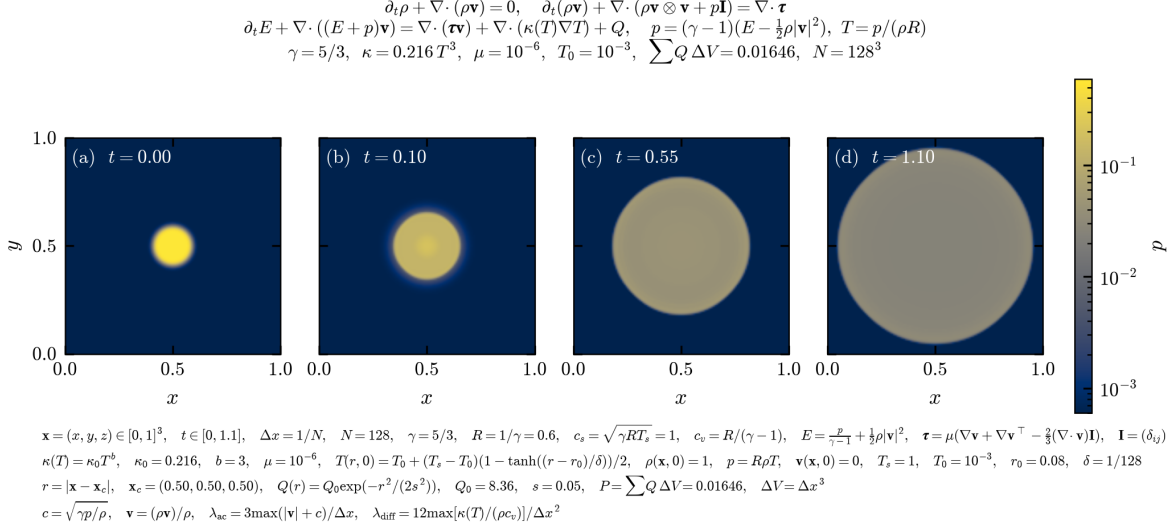
Figure 4: Pressure p on the midplane z = 0.5 of explosion B at times t = 0, 0.10, 0.55 , and 1.10 . Coordinates x, y, z span the unit cube; N = 128 cells per direction. The conductivity is \kappa(T) = 0.216 T^3 , the viscosity is \mu = 10^{-6} , the ambient temperature is T_0 = 10^{-3} , and the ratio of specific heats is \gamma = 5/3 . The color scale is logarithmic.
