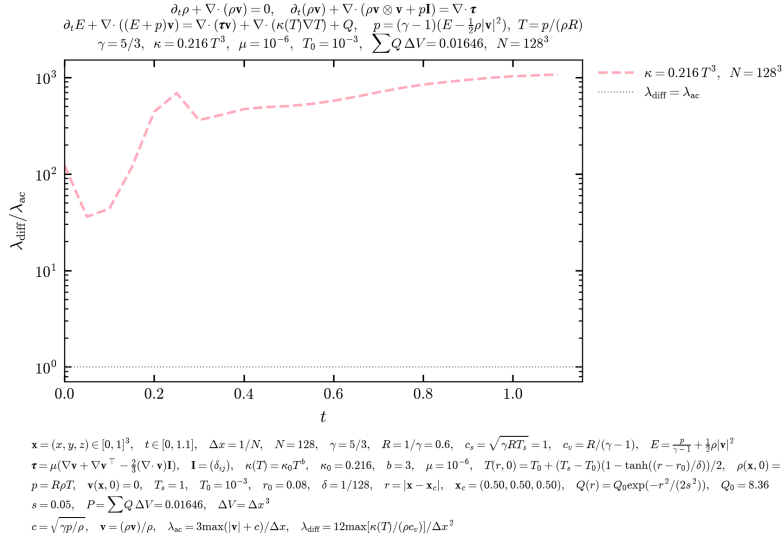
Figure 5: Thermal diffusion-to-acoustic rate ratio \lambda_{diff}/\lambda_{ac} versus time t for explosion B. Here \lambda_{diff} = 12 \max[\kappa(T)/(\rho c_v)]/\Delta x^2 , \lambda_{ac} = 3 \max(|\mathbf{v}| + c)/\Delta x , \Delta x = 1/128 , \rho is density, c_v is the specific heat at constant volume, \mathbf{v} is velocity, and c is the local sound speed. The dotted line marks equal rates.
