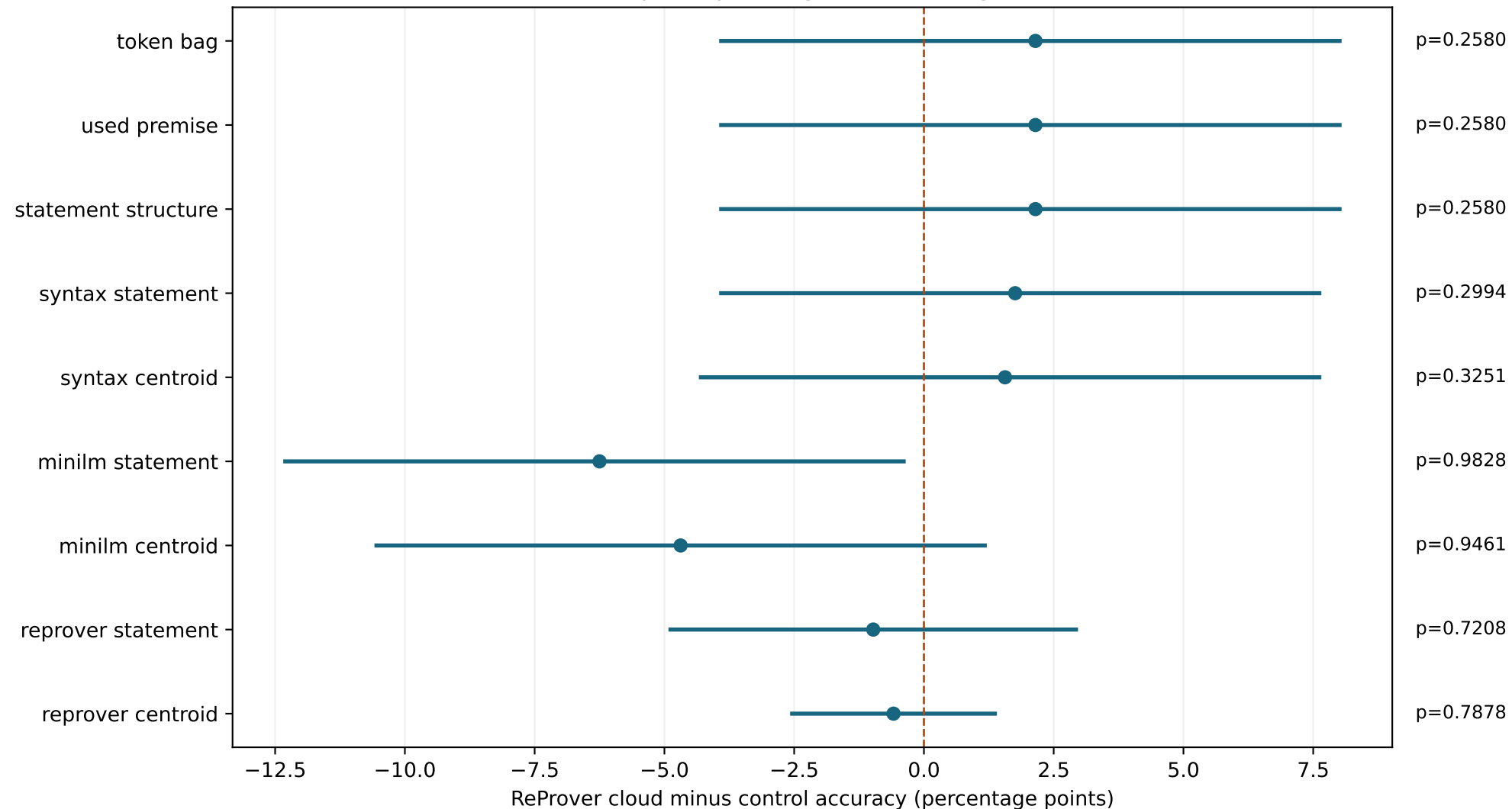
GPU check: 512 triplets, paired gains and marginal 95% intervals
