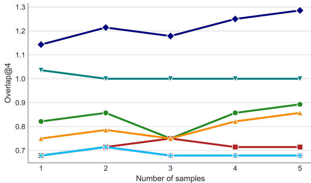
Overlap@4
