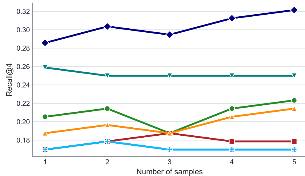
Recall@4
