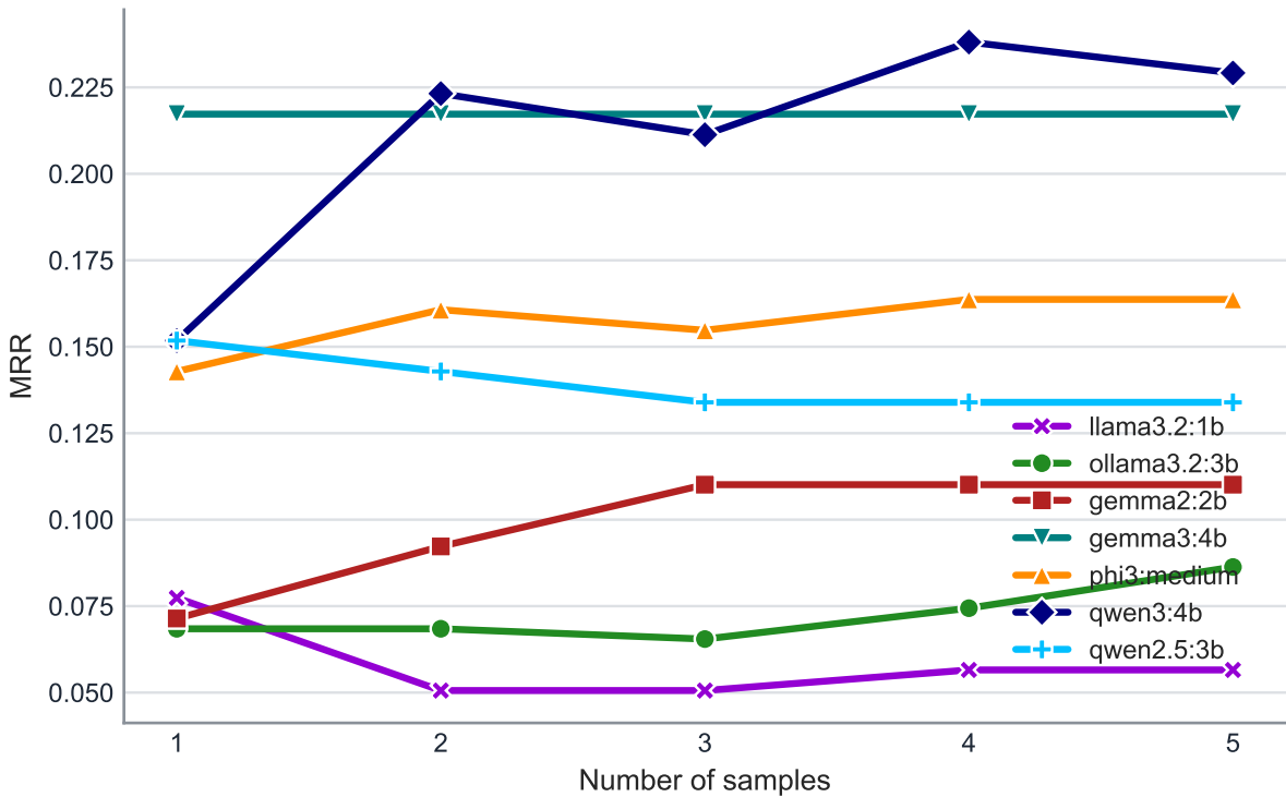
MRR
