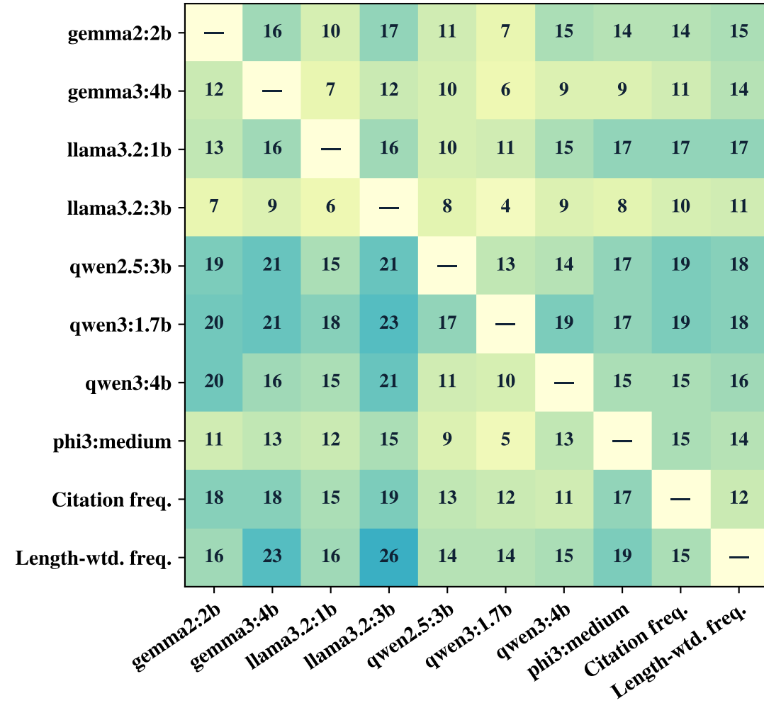
Top-4 Overlap
