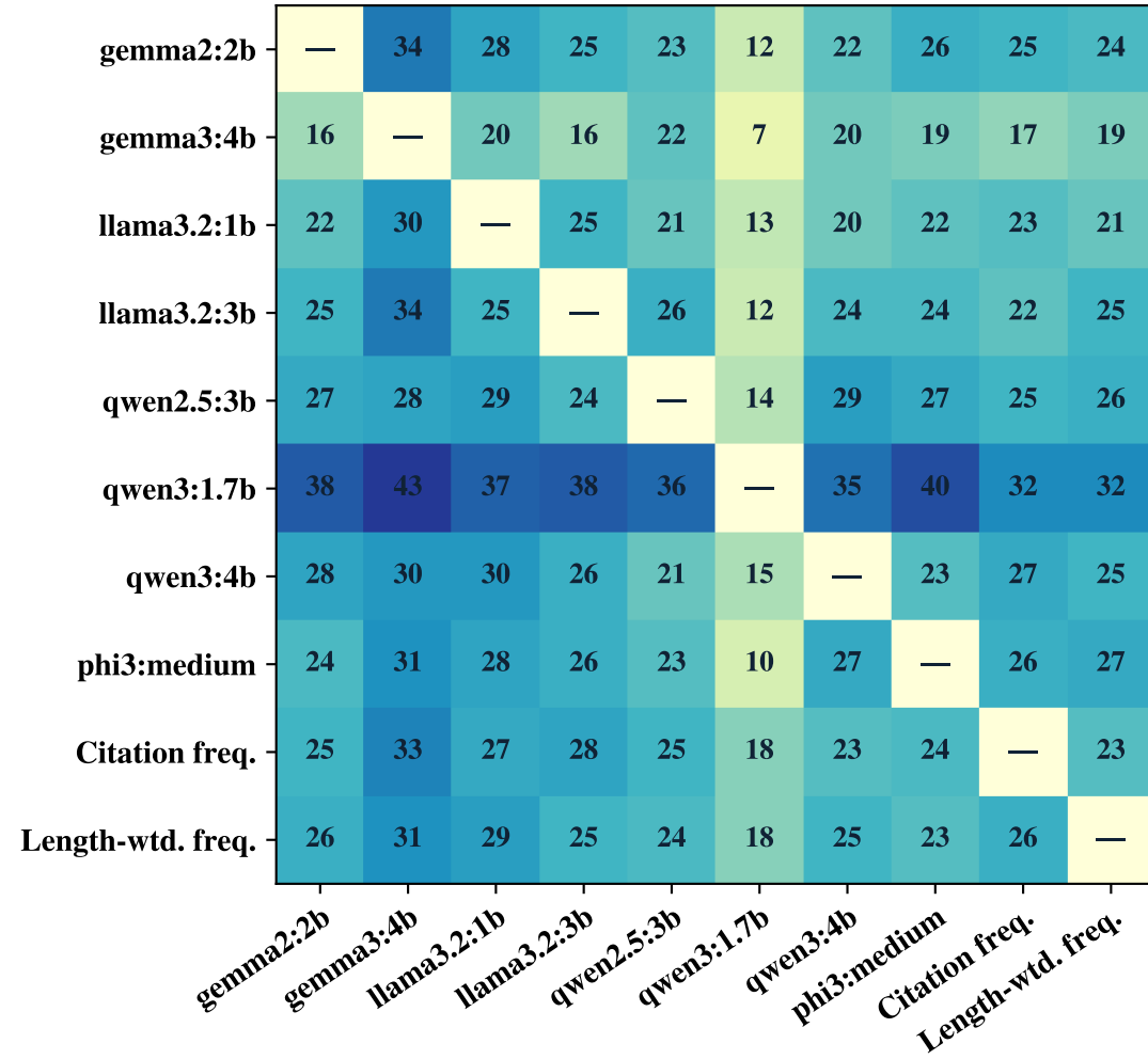
Spearman \rho
