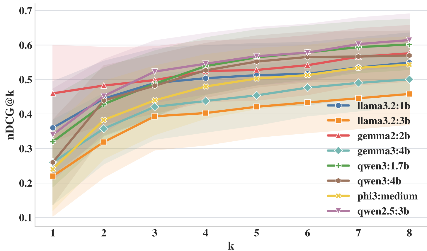
nDCG@k
