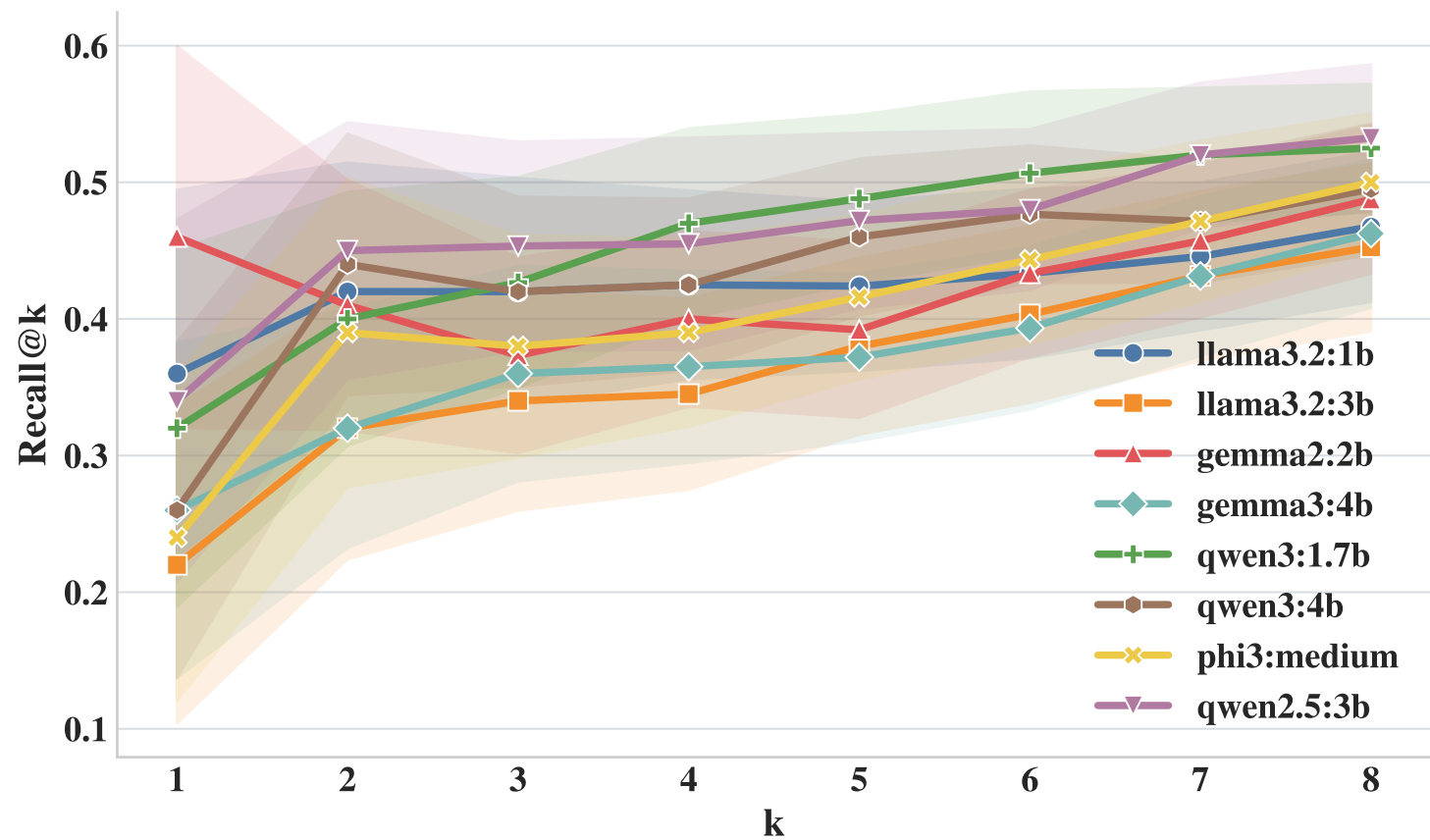
Recall@k
