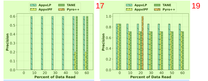
(a) Precision at k = 5 , DB Status (b) Precision at k = 7 for Letter Figure 2: Precision for top- k AFDs with l = 3 when data is indexed by key like attributes
