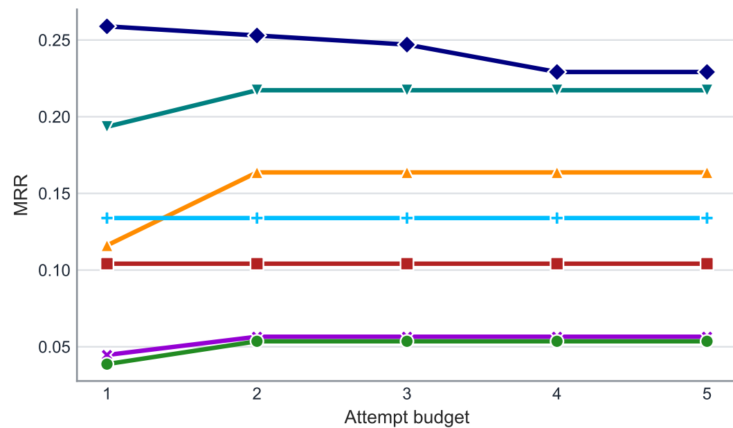
MRR
