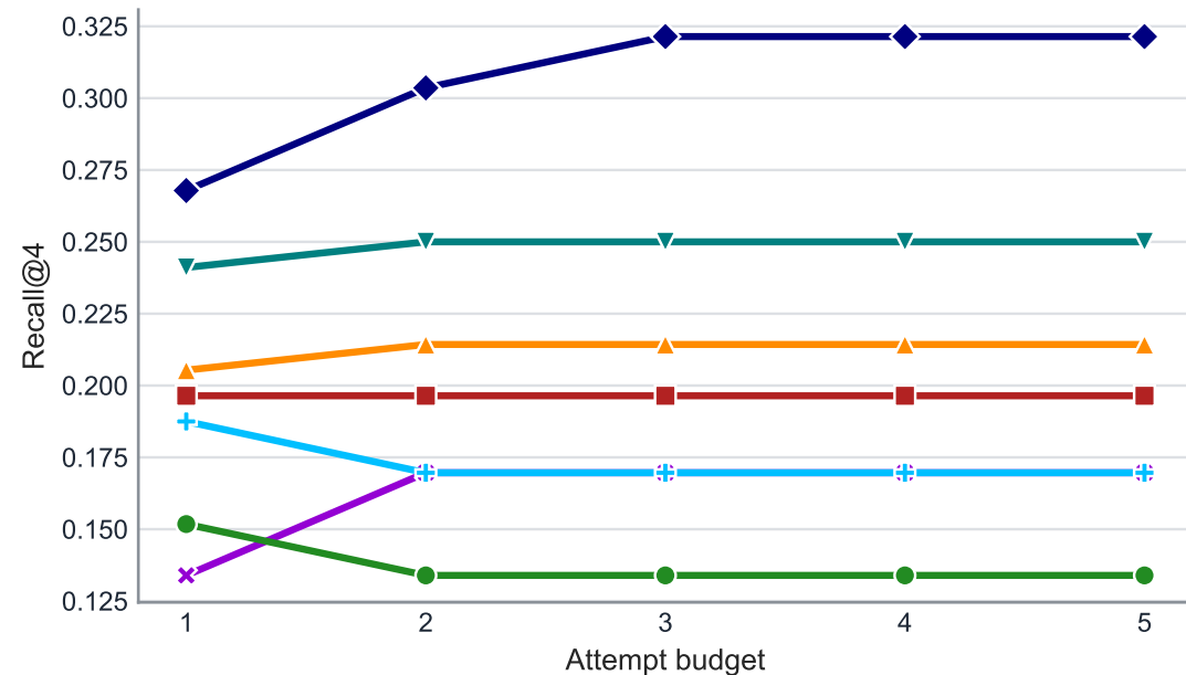
Recall@4
