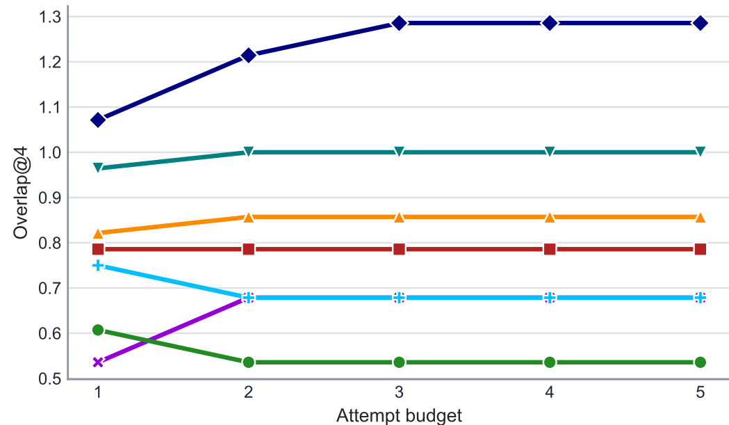
Overlap@4
