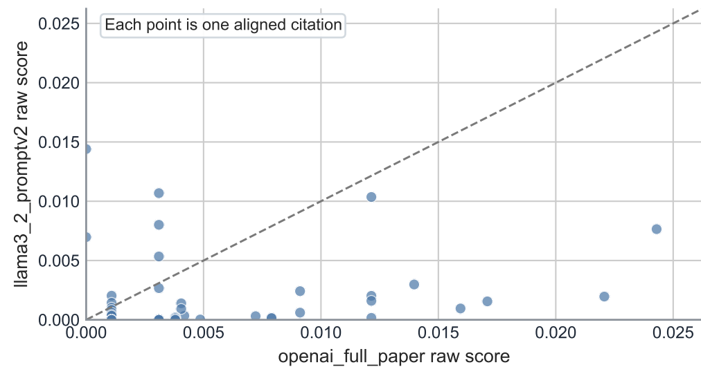
Raw Citation Scores
