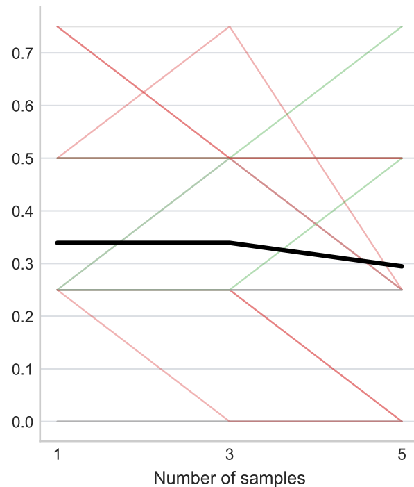
Recall@4
