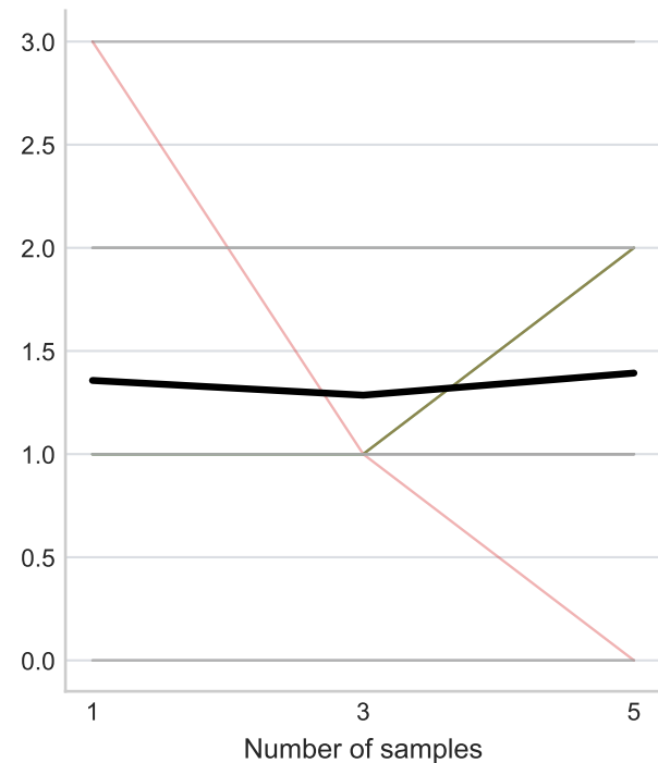
Overlap@4
