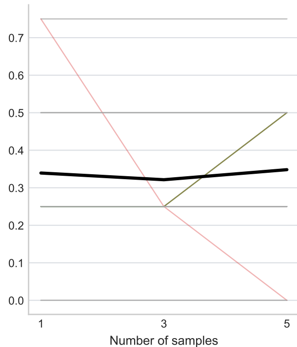
Recall@4
