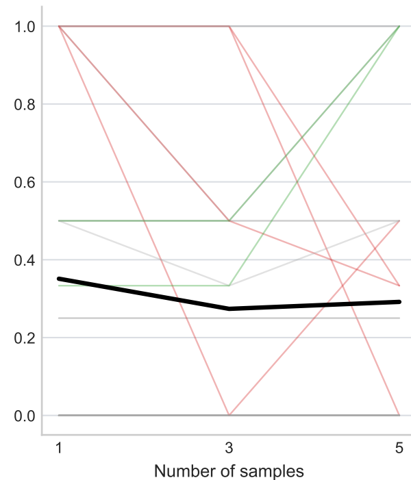
MRR
