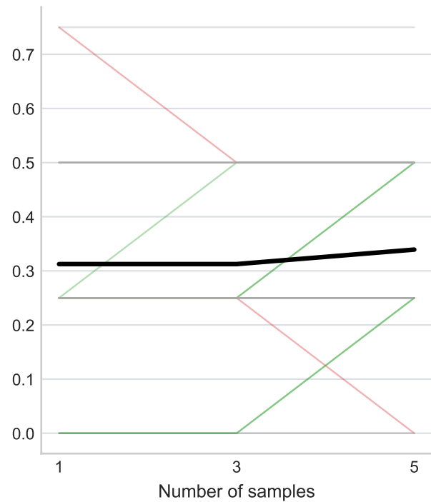
Recall@4
