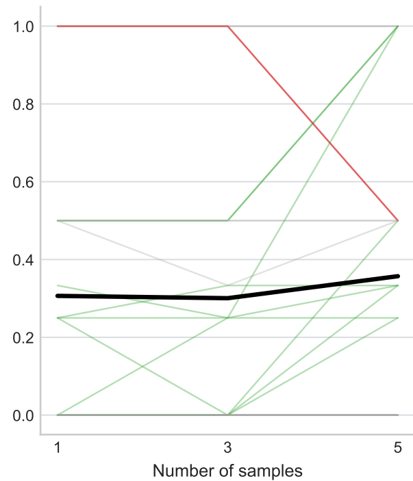
MRR
