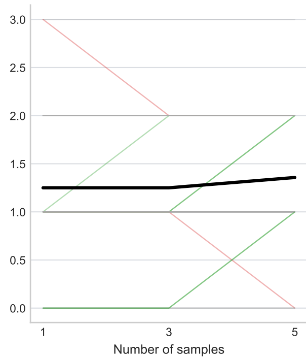
Overlap@4
