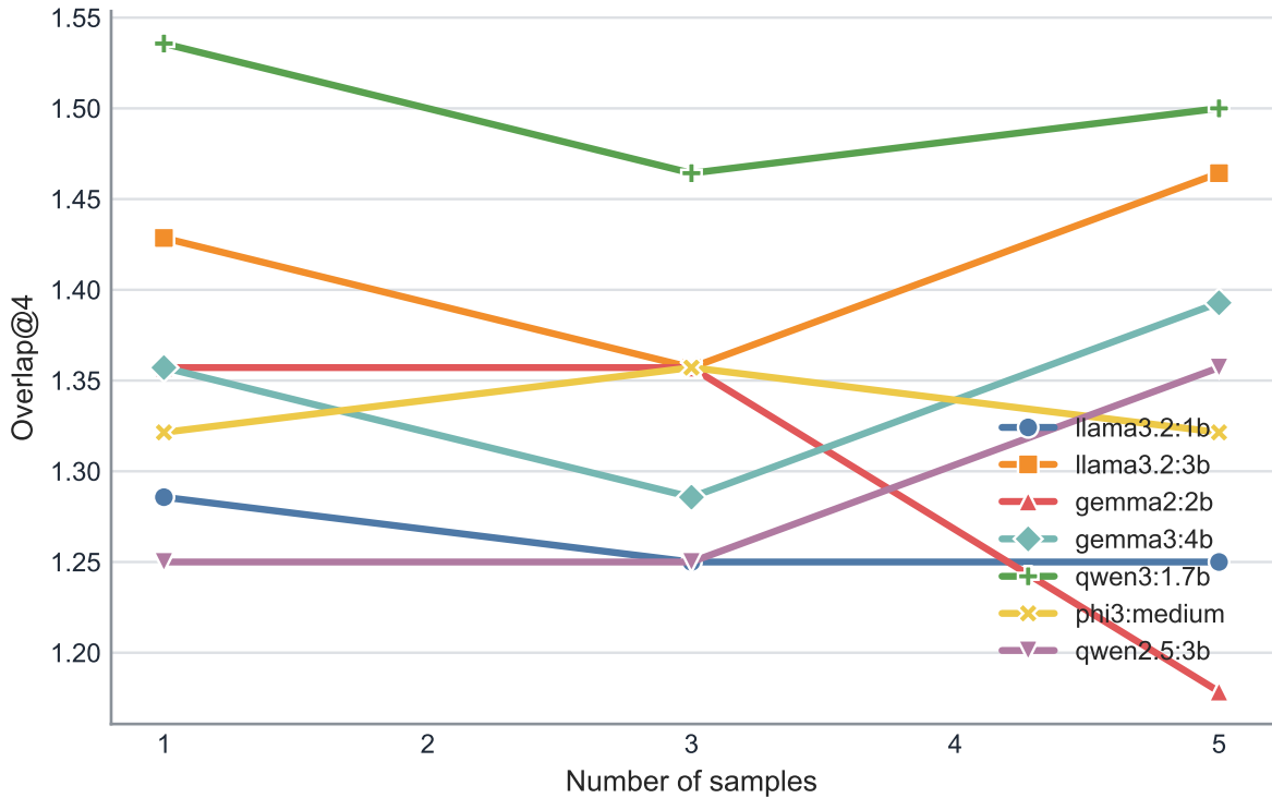
Overlap@4
