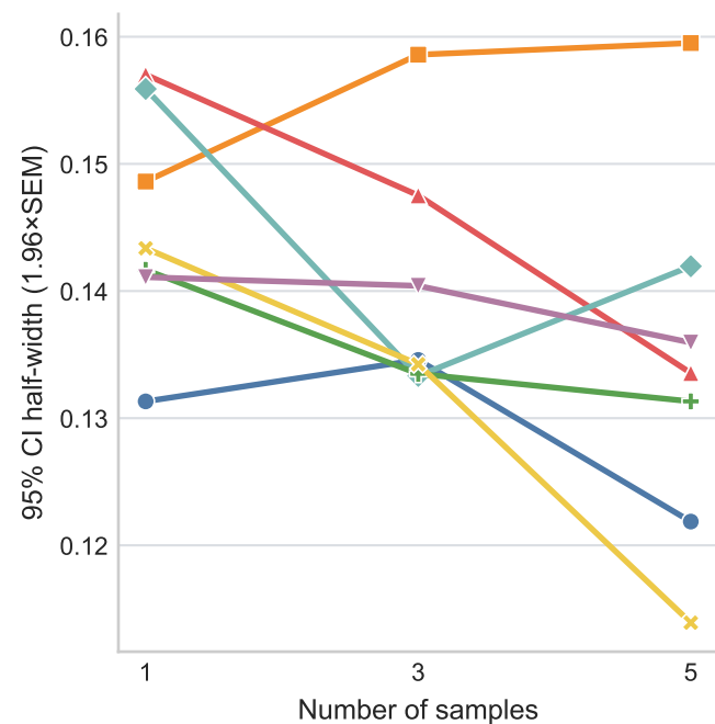
MRR
