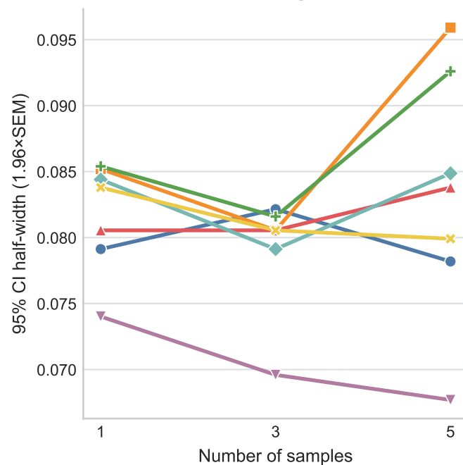
Recall@4
