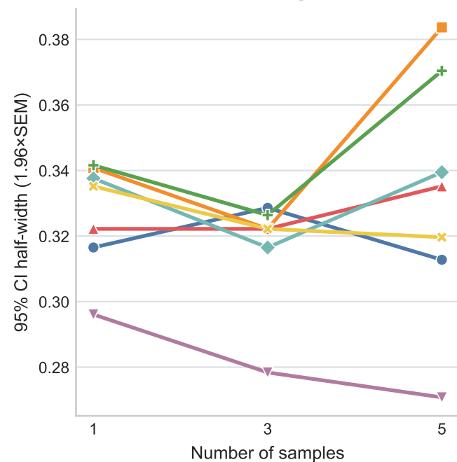
Overlap@4
