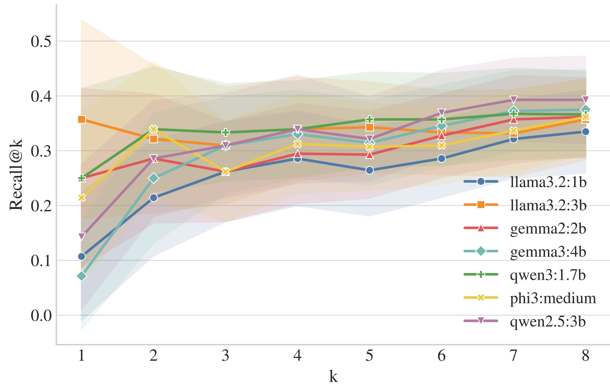
Recall@k
