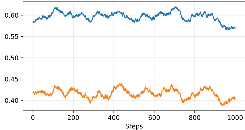
Stage 2: scale_mean
