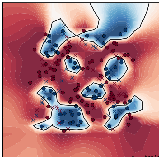
Checkerboard
