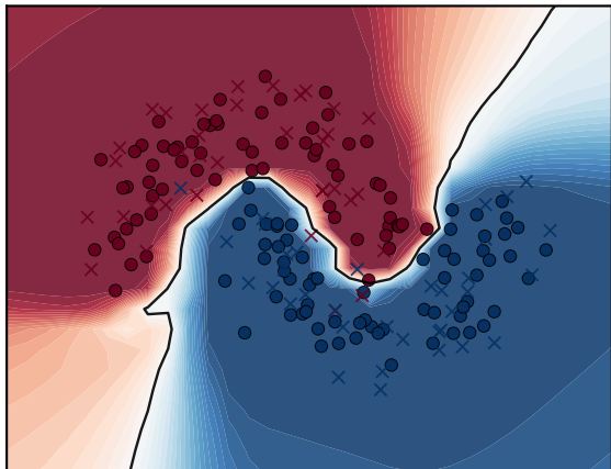
TabICL + PDL head
