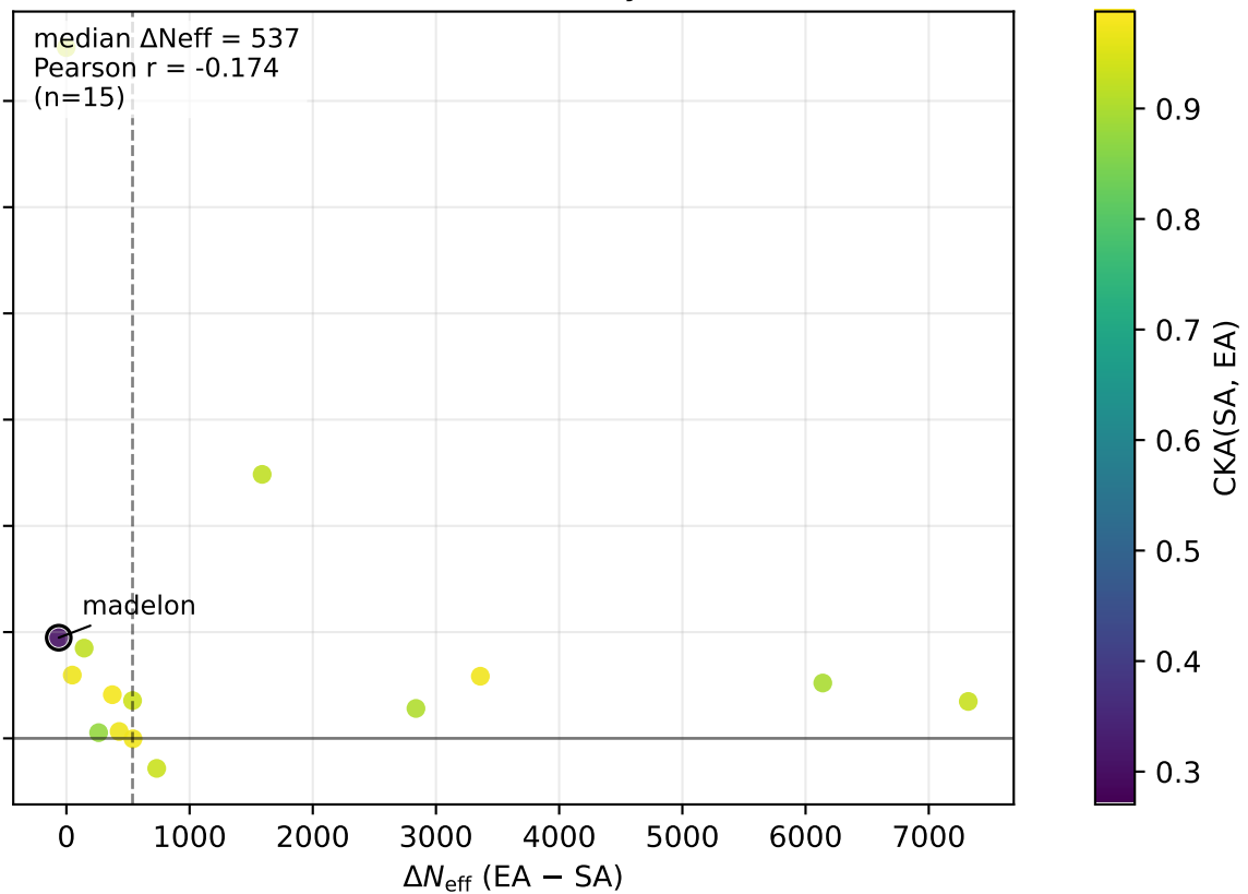
EA-ICL (ICL only)
