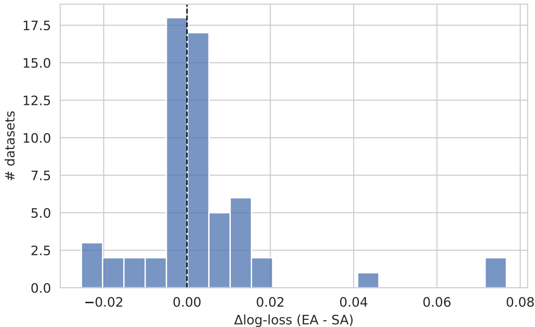
CC18 per-dataset \Delta\log\text{-loss}
