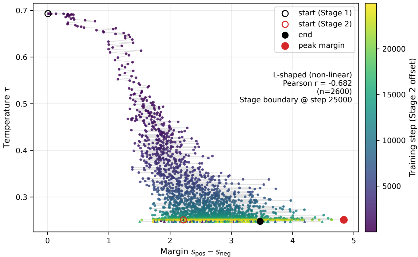
Automatic temperature scaling vs. learned margin (full run)
