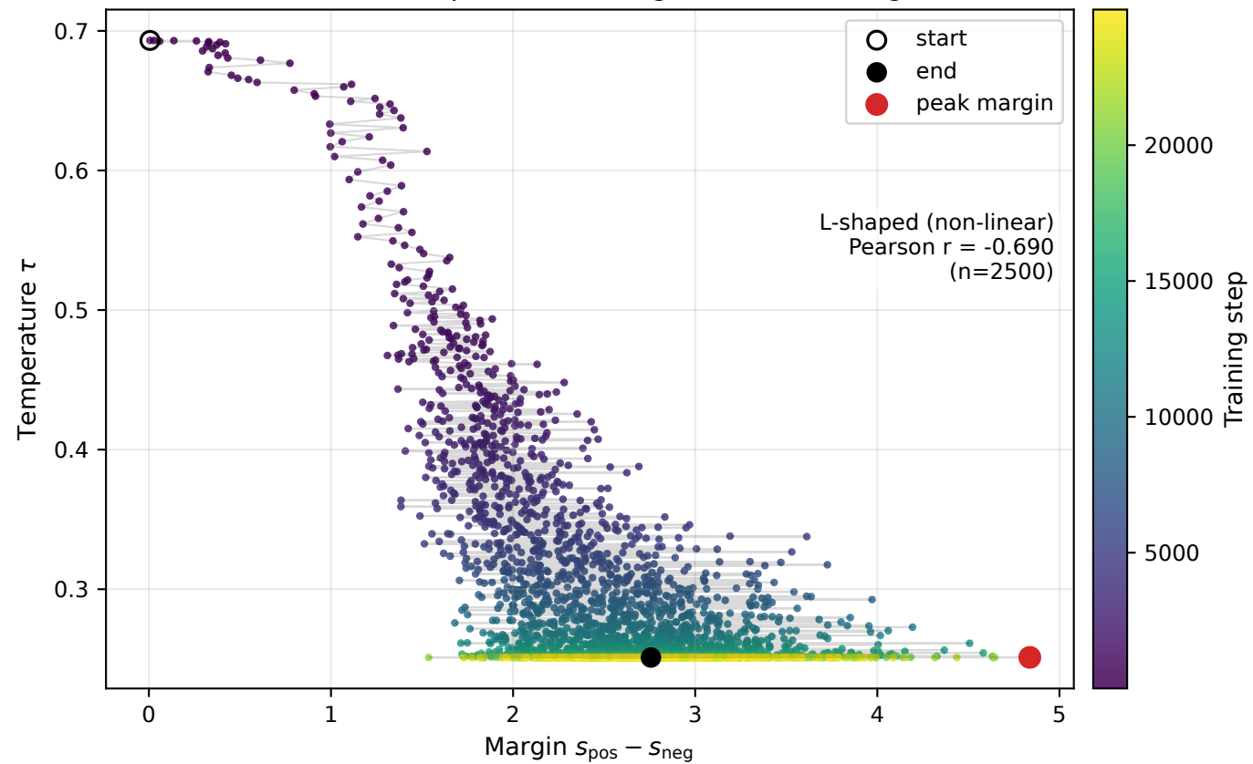
Automatic temperature scaling vs. learned margin
