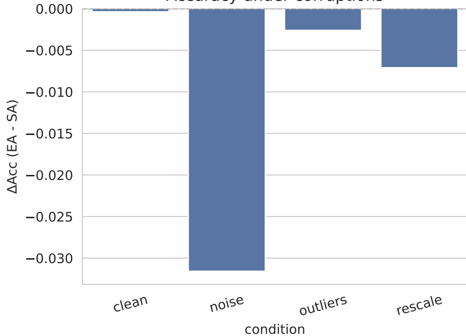
Accuracy under corruptions
