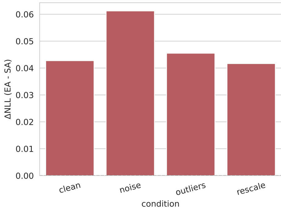
Log-loss under corruptions
