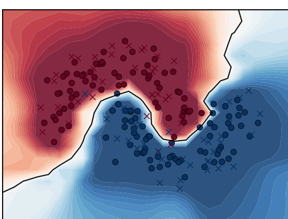
Two Moons
