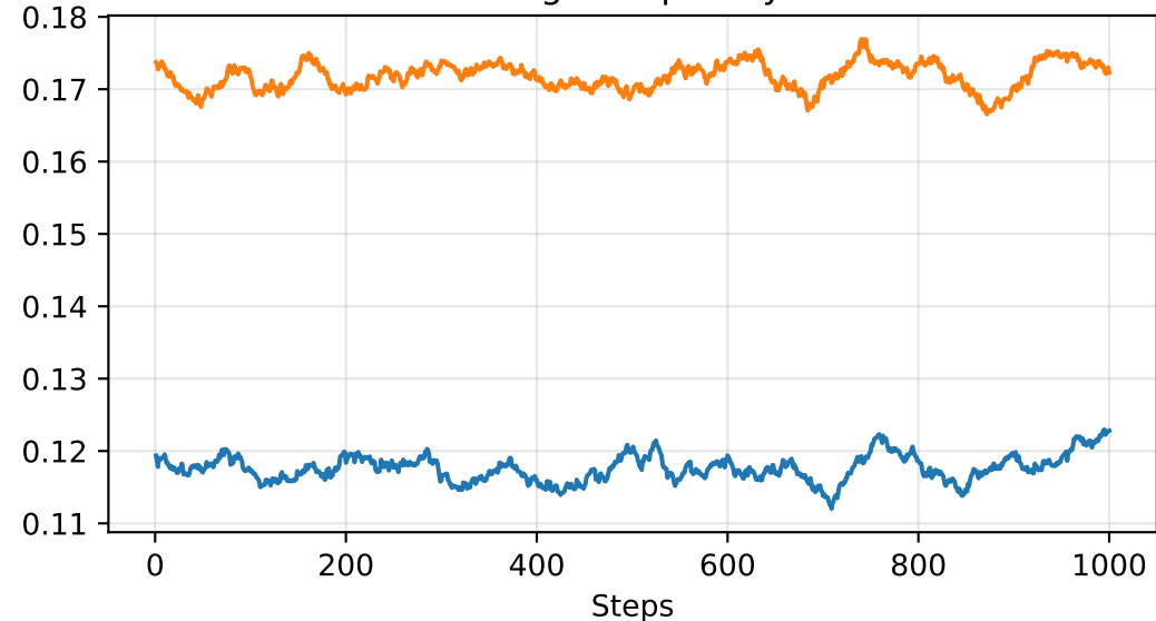
Stage 2: scale_mean
