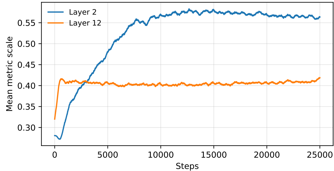
Stage 1: scale_mean
