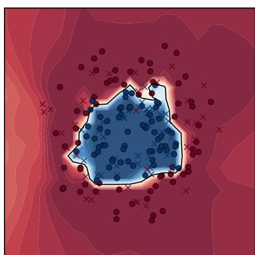
Circles
