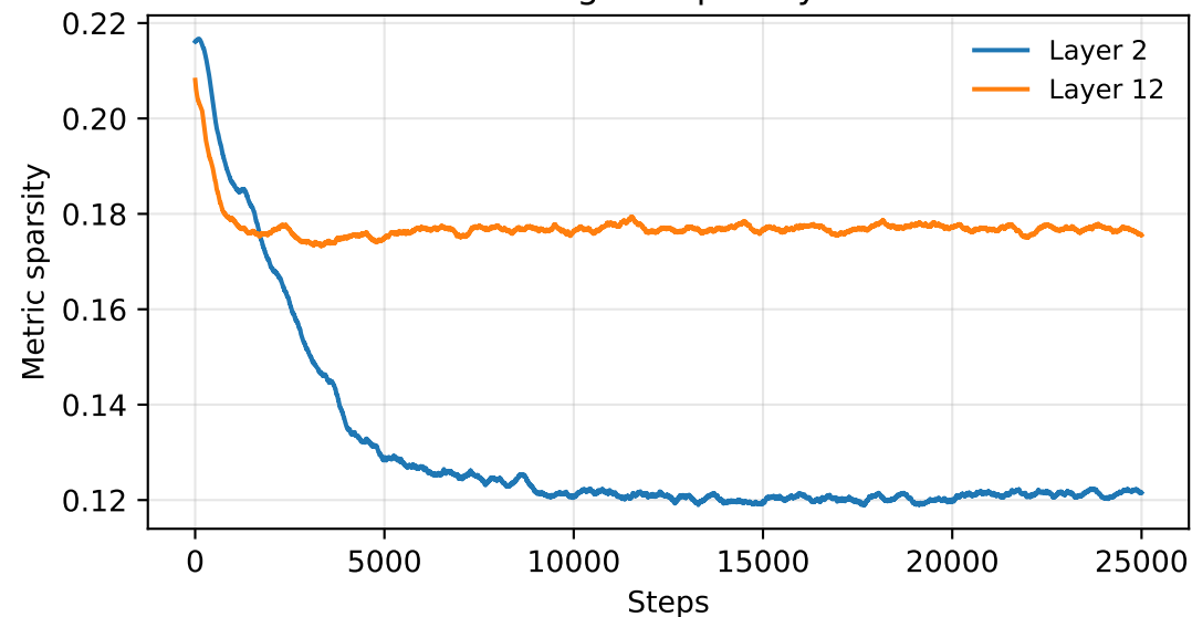
Stage 1: scale_mean
