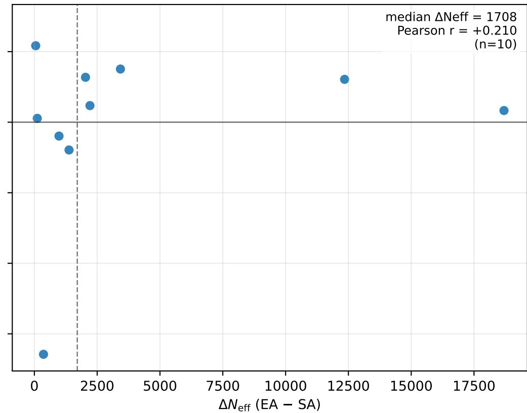
EA-ICL ( \text{TF}_{\text{icl}} )
