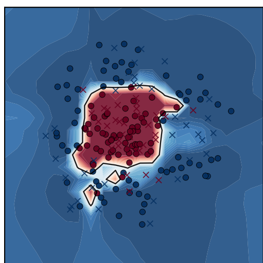
Ring
