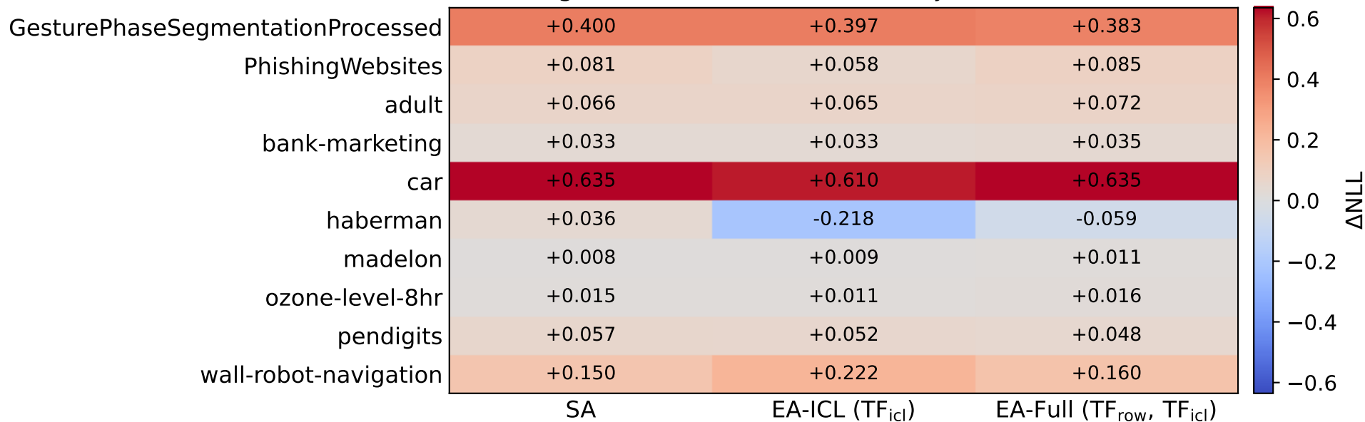
NLL change: Uninformative feature injection ( k = 50 ) – Clean
