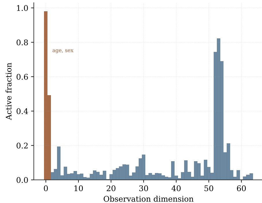
(a) 64-dim feature activation frequency
