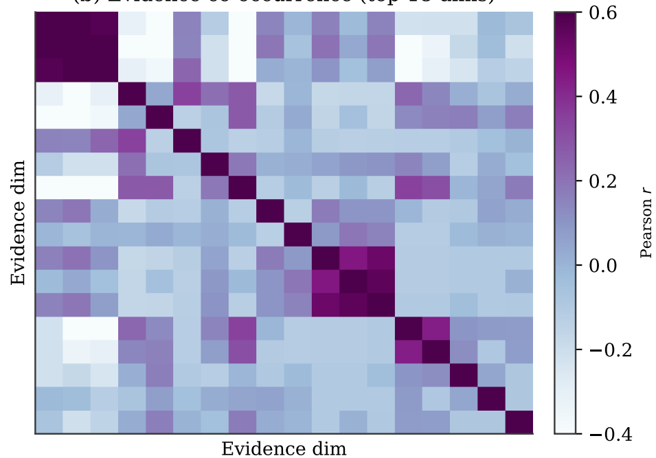
(b) Evidence co-occurrence (top-18 dims)
