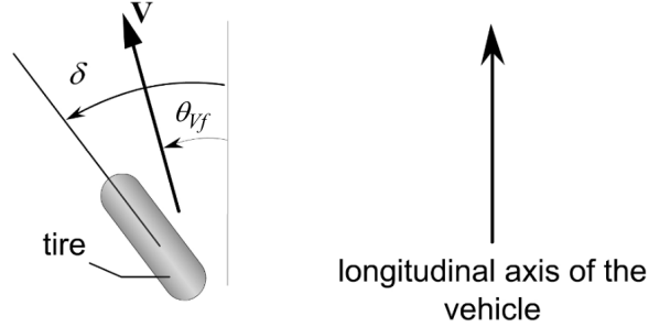
Figure 2: Tire slip angle [2]
