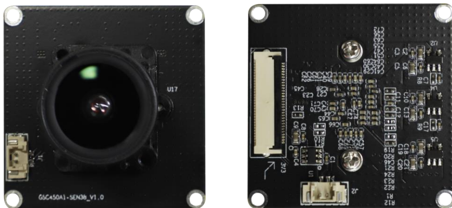
GSC450AI-SEN38 Sensor 板正反面图
