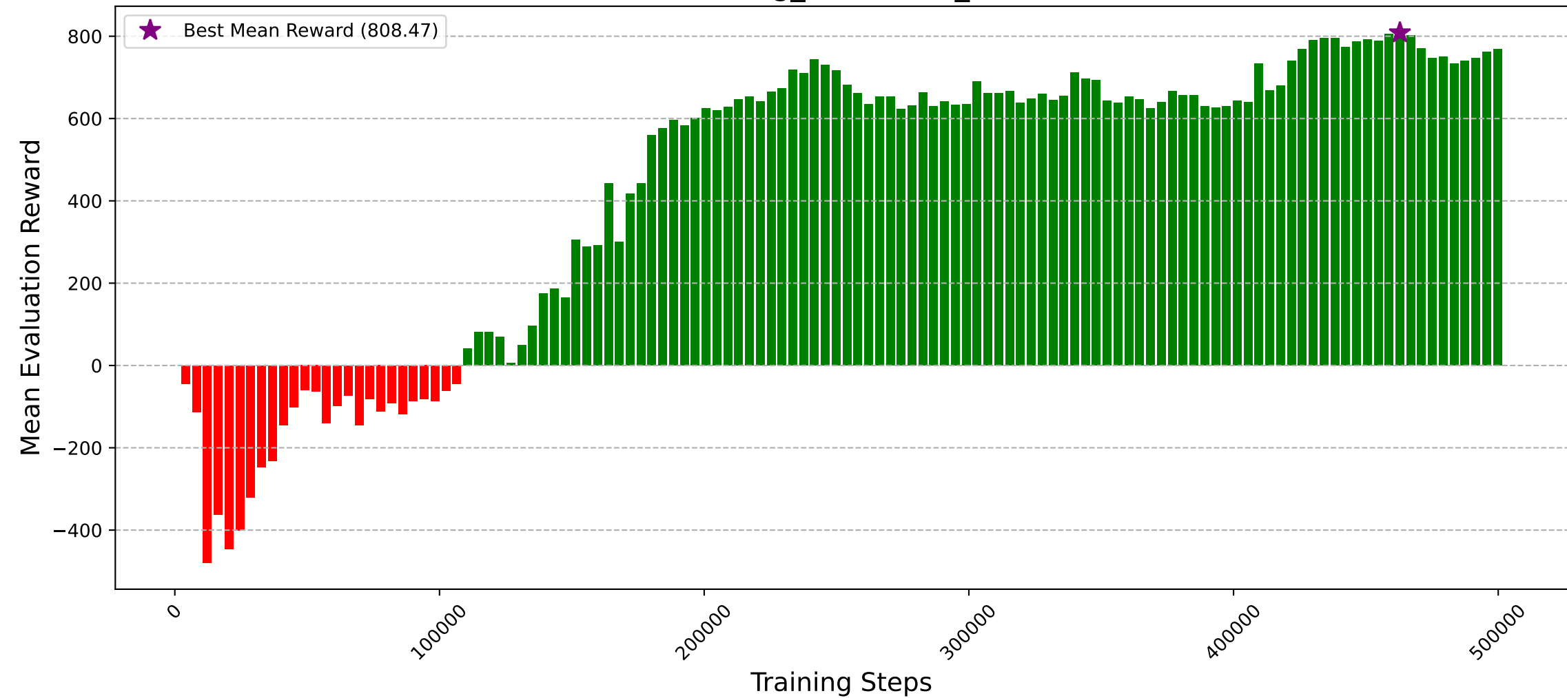
Mean Evaluation Reward vs Training Steps (Run: training_20250328_131443)
