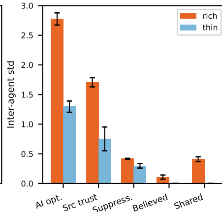
(c) Stance Probe Divergence
