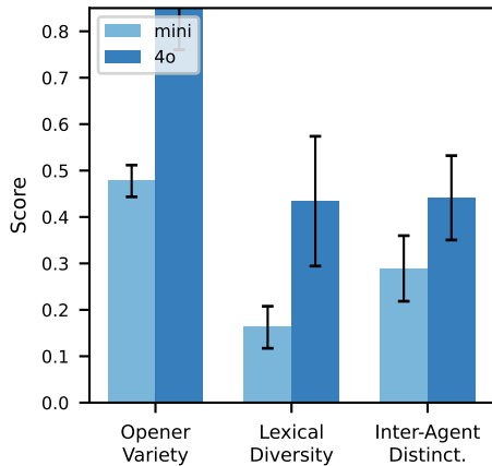
(a) Model Capacity
