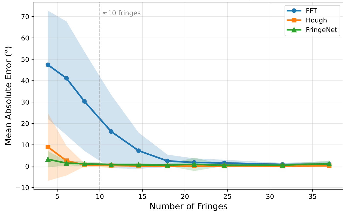
Orientation Estimation Error vs Fringe Density
