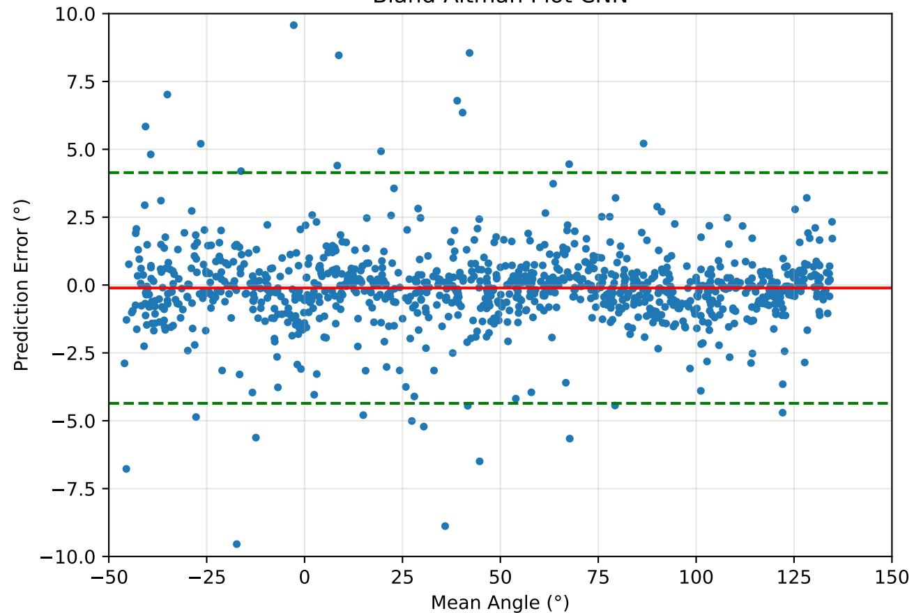
Bland-Altman Plot CNN
