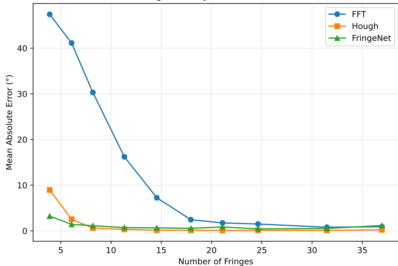
Effect of Fringe Density on Orientation Estimation
