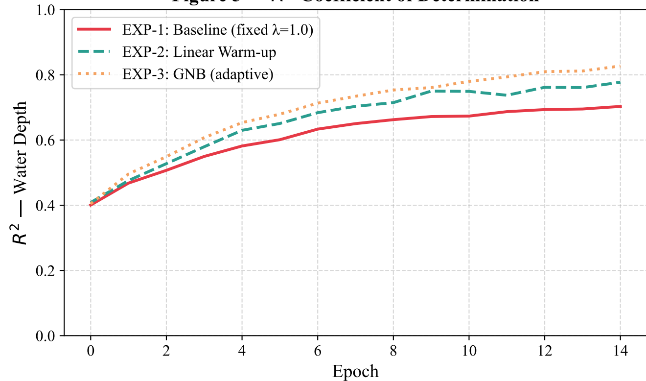
Figure 5 — R^2 Coefficient of Determination
