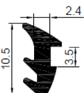
Cap Gasket (Skirting) CODE: MP-2020
