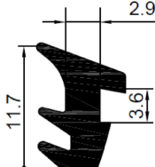
Half Bubble Seal CODE: MP-2023
