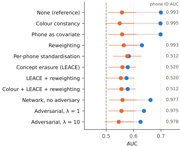
B Shortcut mitigation (DINOv2 features)
