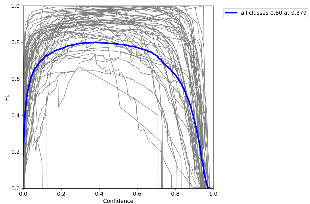
Figure 7-10. F1 Score-Confidence Curve for YOLOv7
