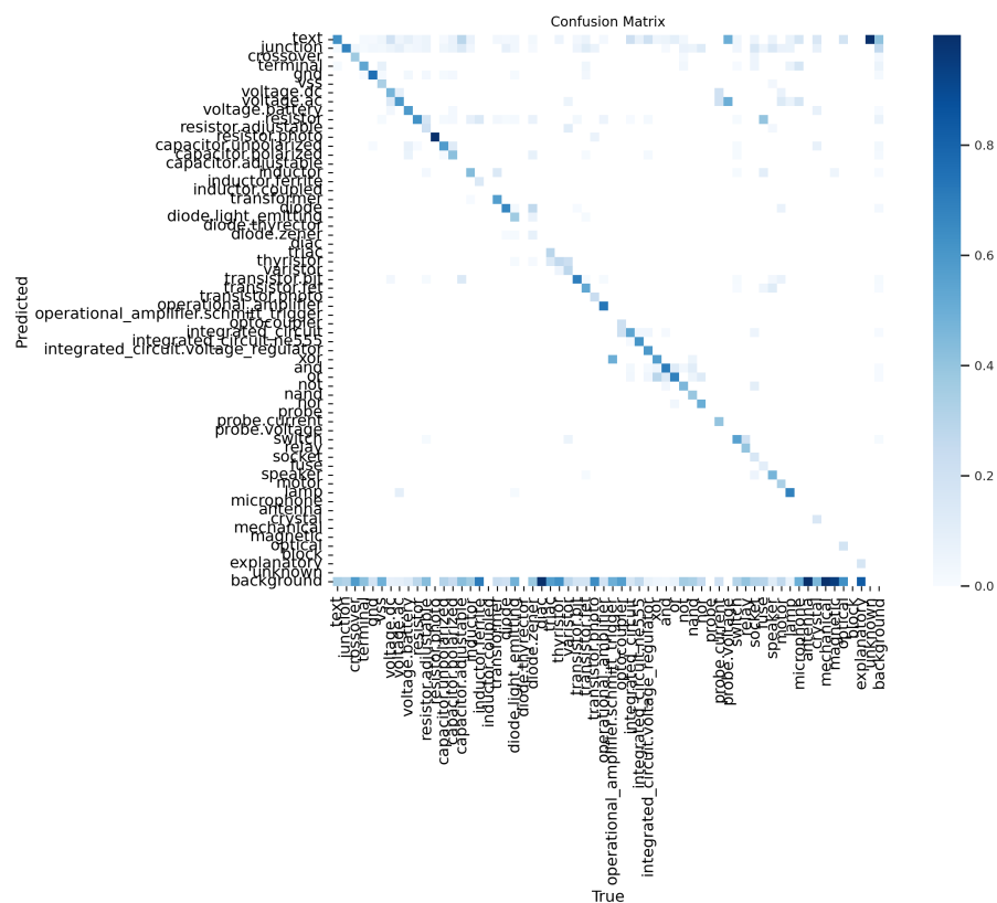
Figure 7-13. Confusion Matrix for YOLOv5
