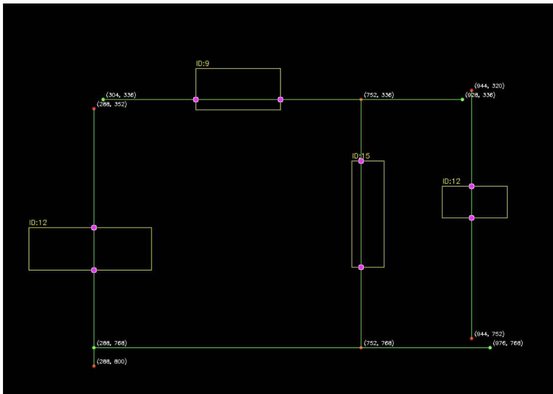
Figure 7-24. Wire-Component Intersection Detection
