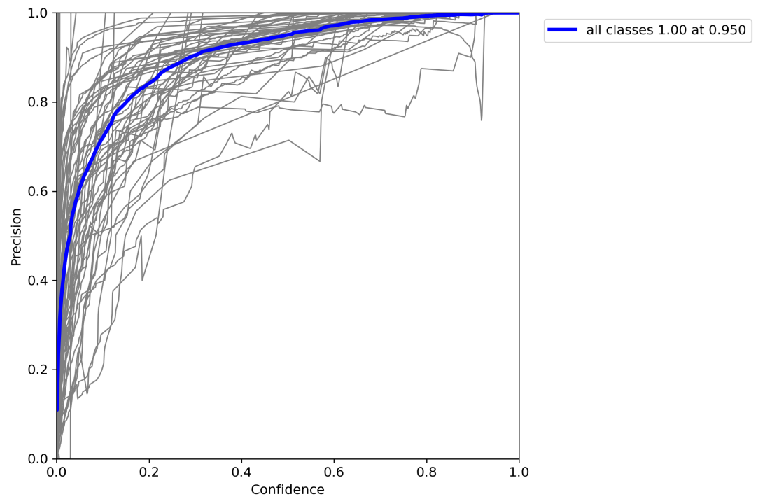
Figure 7-6 Precision-Confidence Curve for YOLOv7
