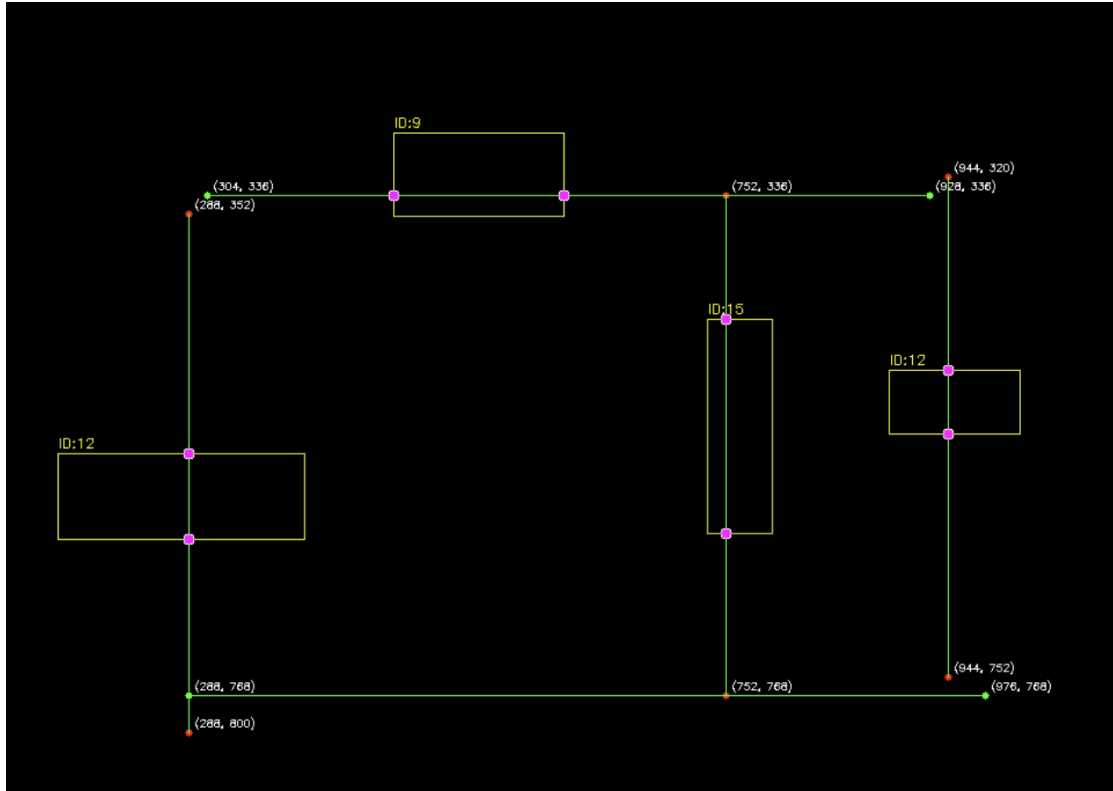
Figure 7-24 Wire-Component Intersection Detection
