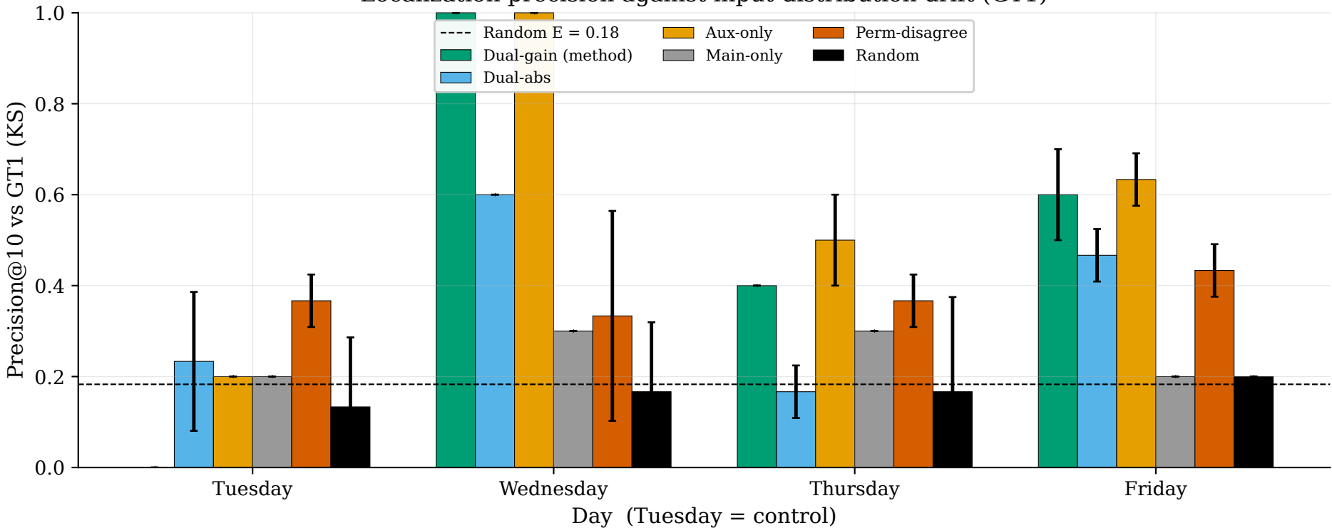
Localization precision against input-distribution drift (GT1)
