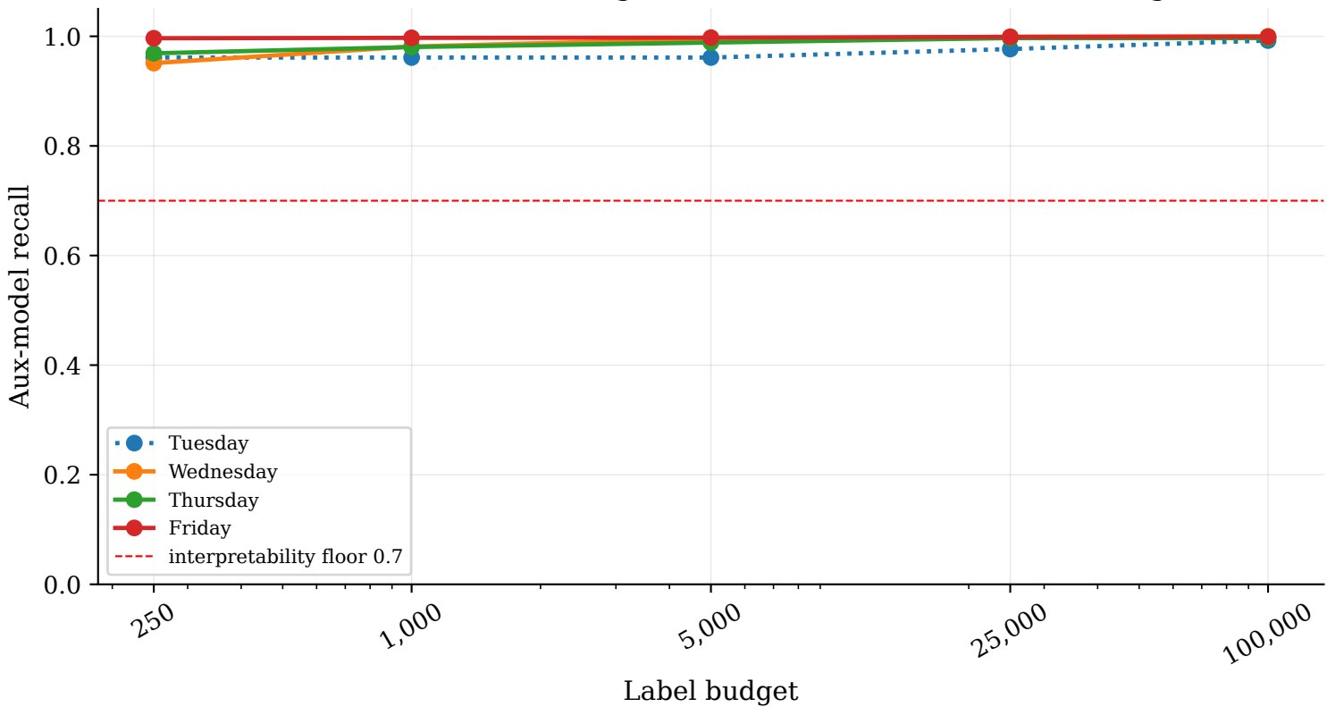
Aux-model recall vs label budget (below the floor, SHAP is meaningless)
