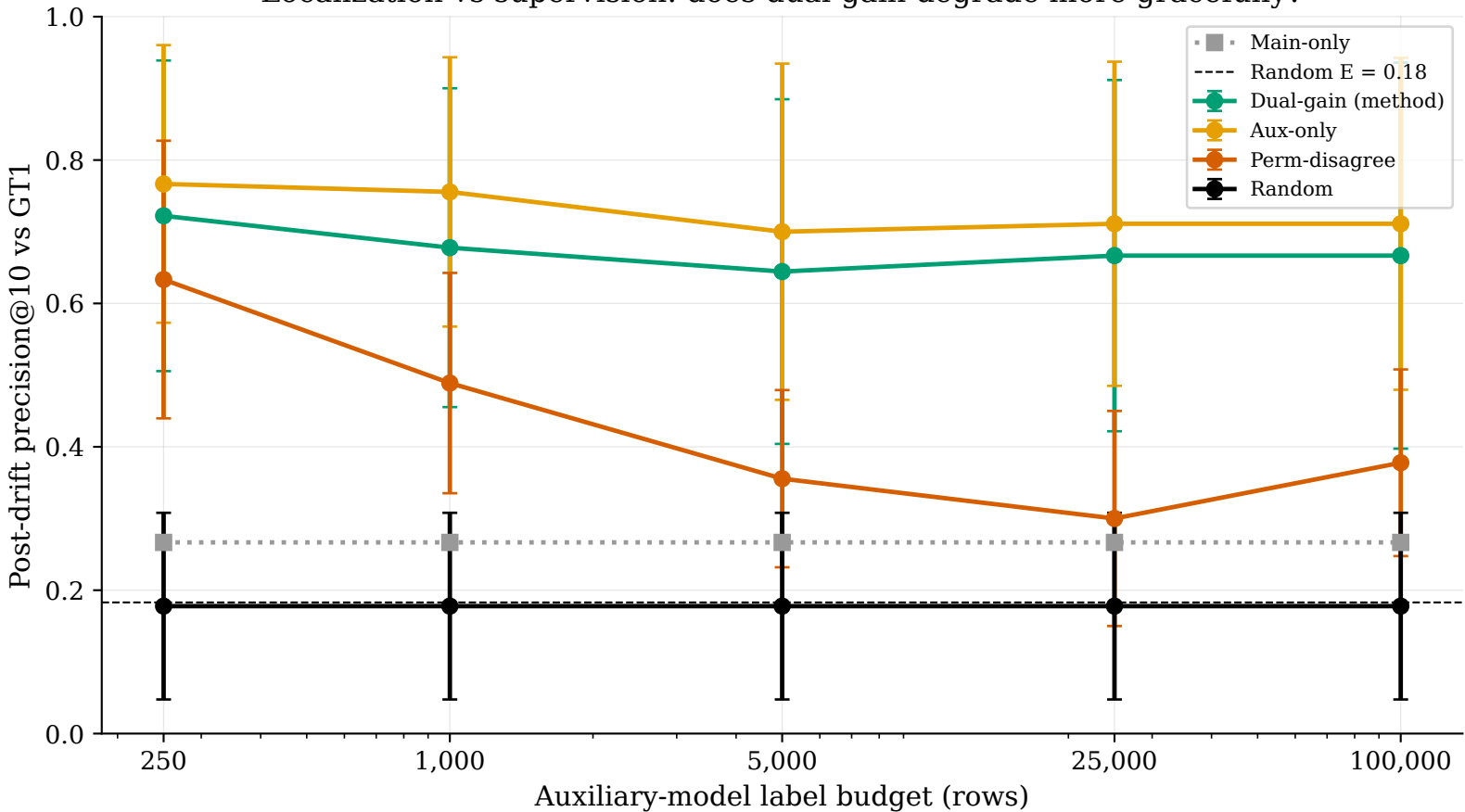
Localization vs supervision: does dual-gain degrade more gracefully?
