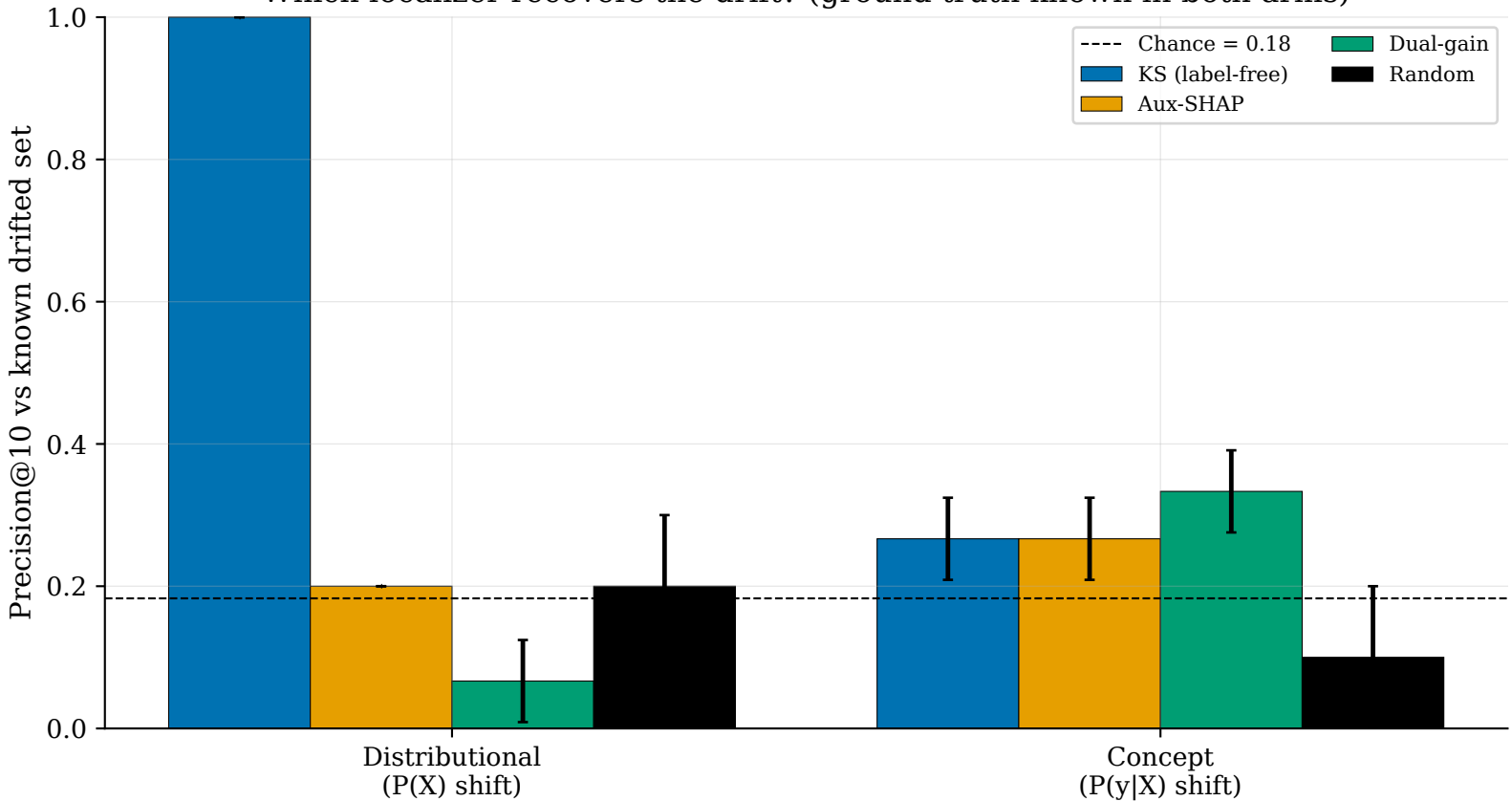
Which localizer recovers the drift? (ground truth known in both arms)
