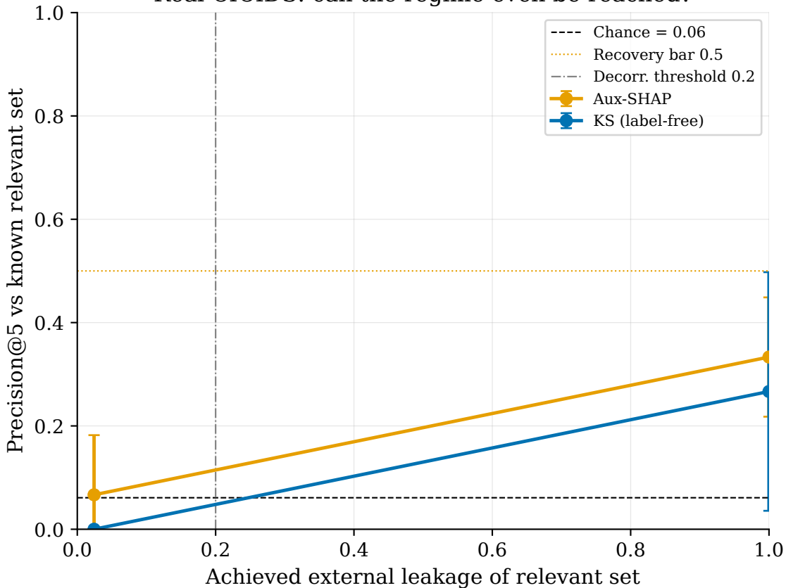
Real CICIDS: can the regime even be reached?
