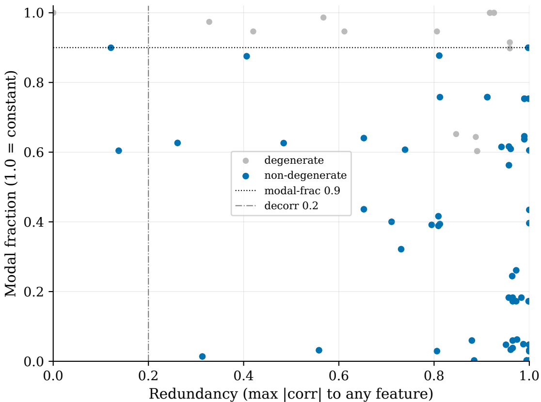
The confound: decorrelated features are near-constant
