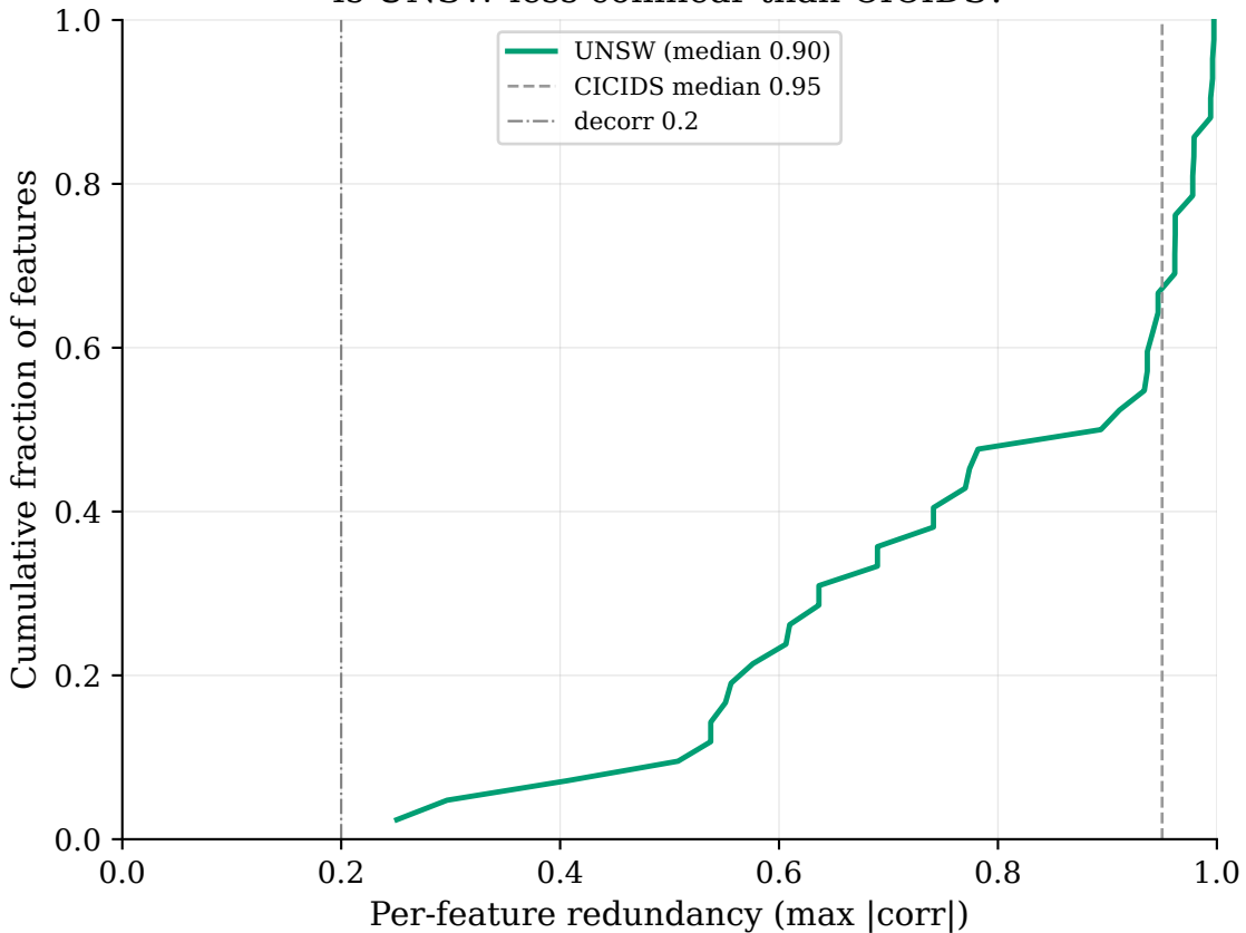
Is UNSW less collinear than CICIDS?
