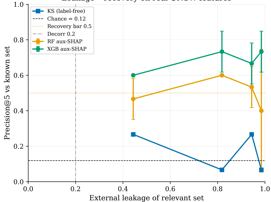
Leakage-&gt;recovery on real UNSW features
