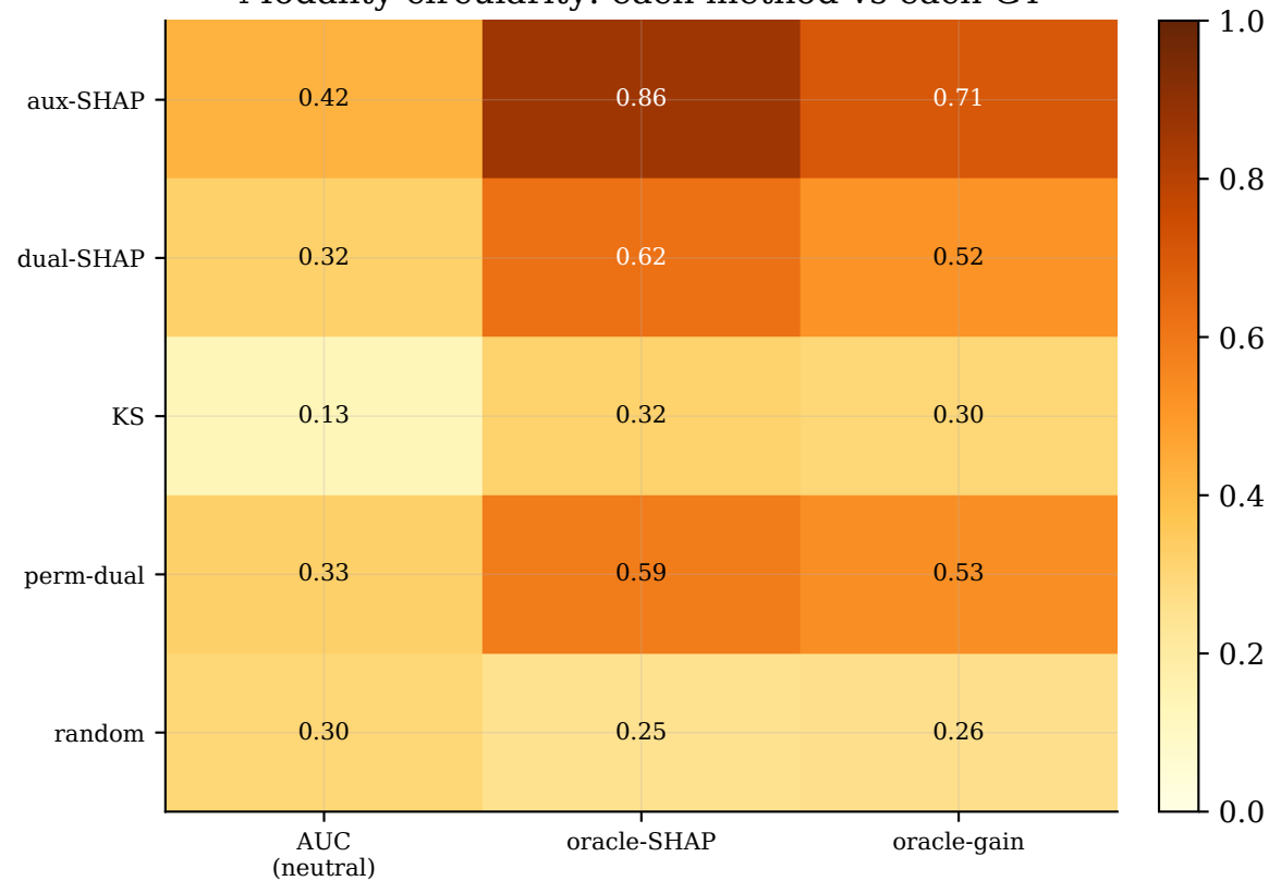
Modality-circularity: each method vs each GT
