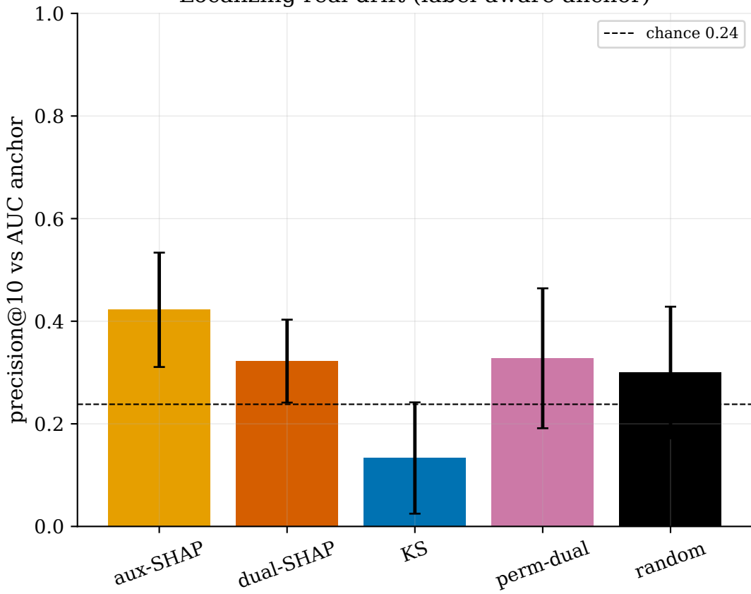
Localizing real drift (label-aware anchor)
