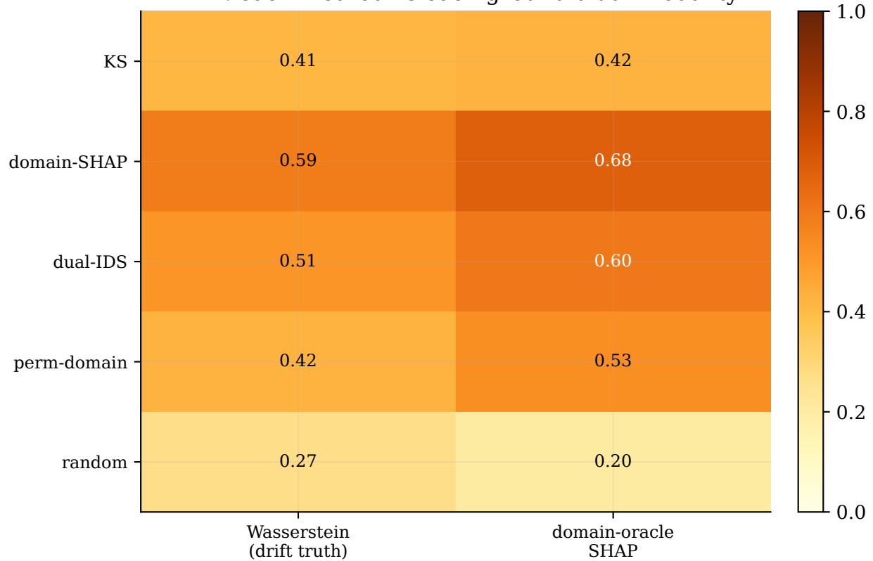
MLP: each method vs each ground-truth modality
