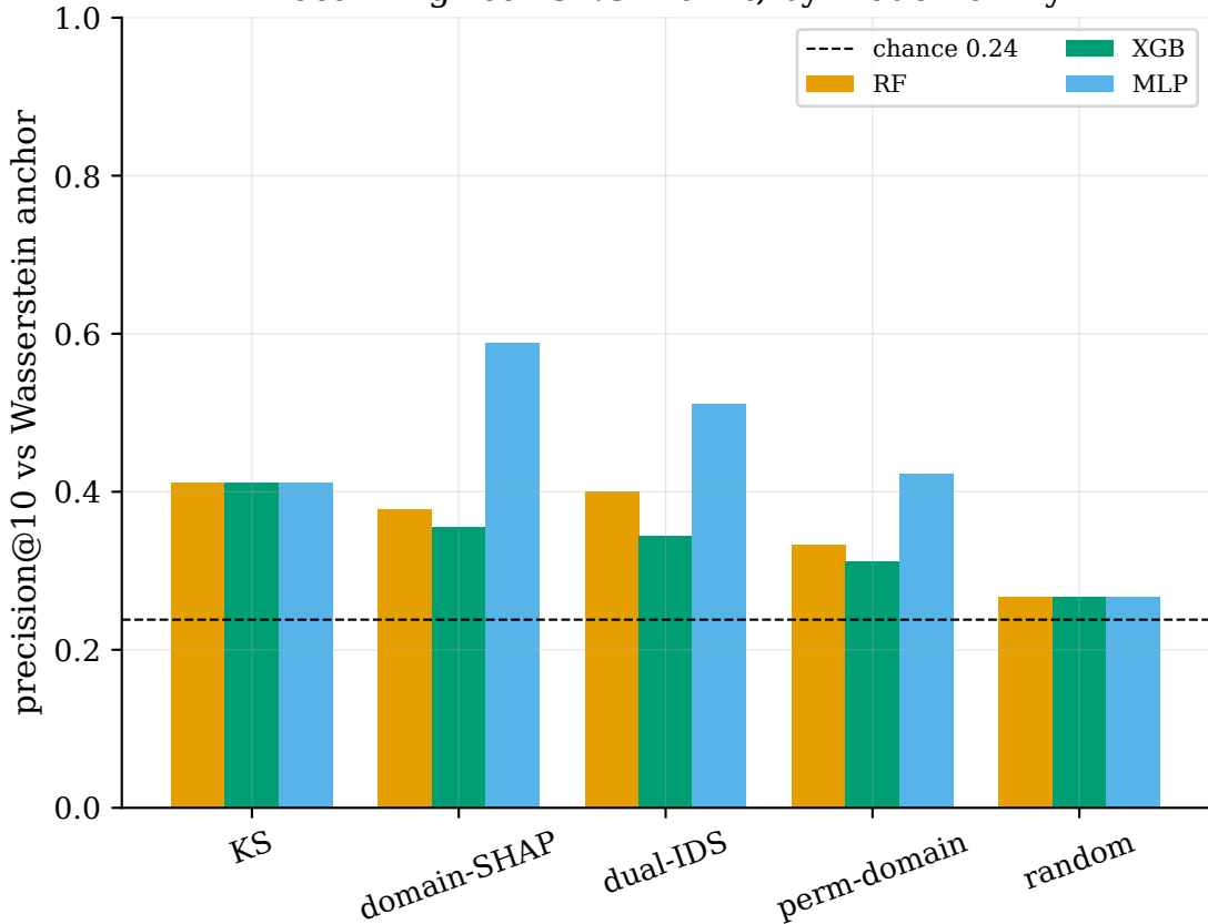
Localizing real UNSW drift, by model family
