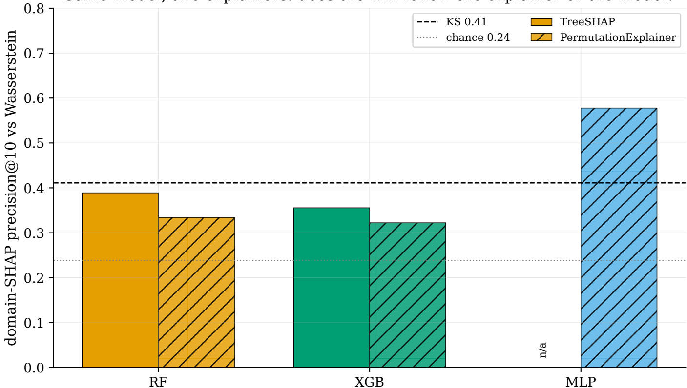
Same model, two explainers: does the win follow the explainer or the model?
