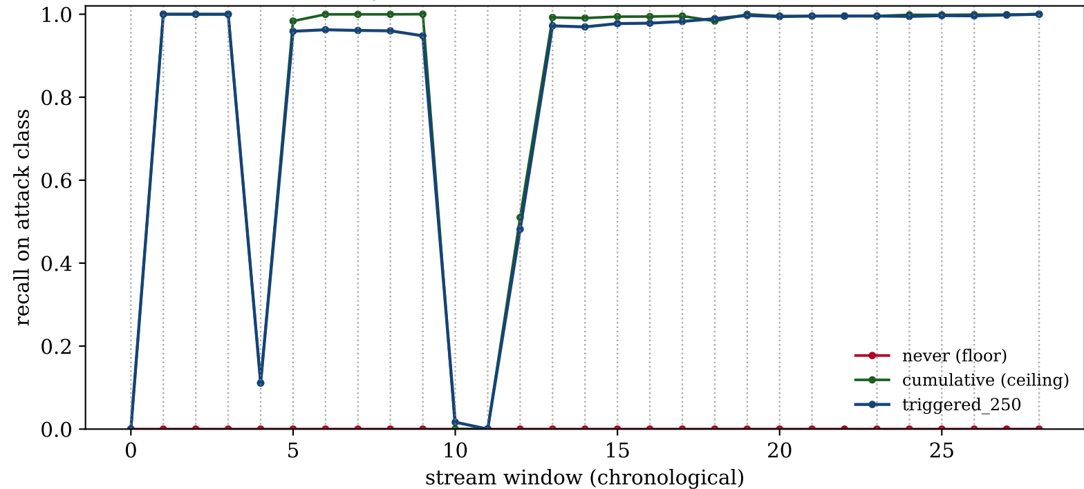
Adaptation trajectories — ADAPTATION-LOOP-CHECK-FAILED
