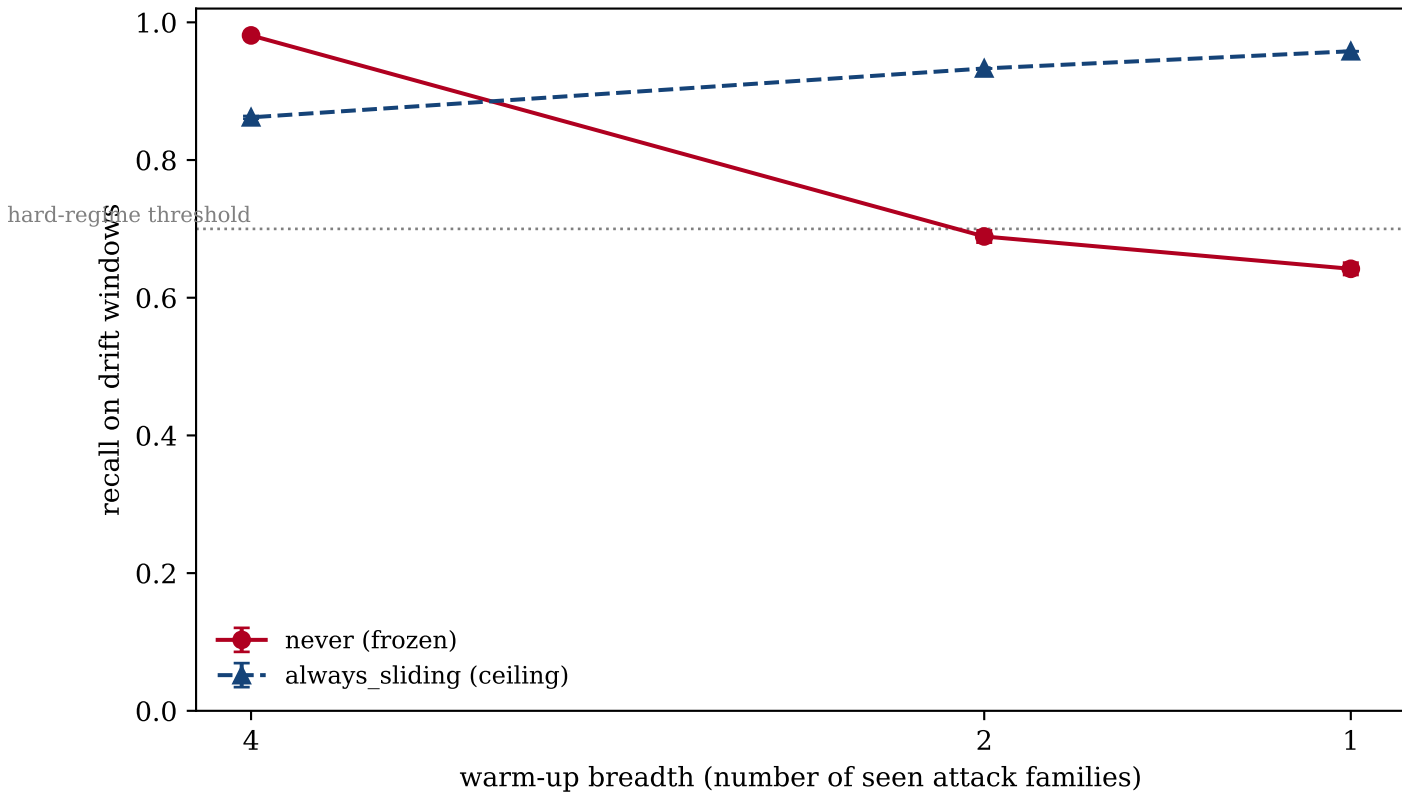
UNSW regime knob, 4 seeds — REGIME-DEPENDENCE-CONFIRMED
