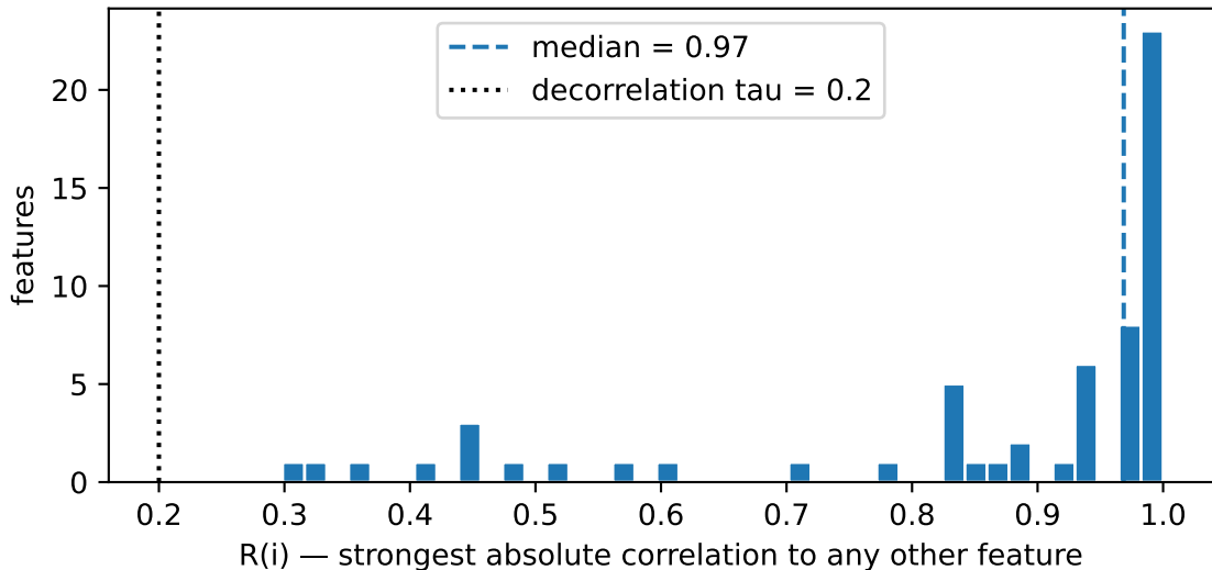
CSE-CIC-IDS2018: feature redundancy (Def. 1)
