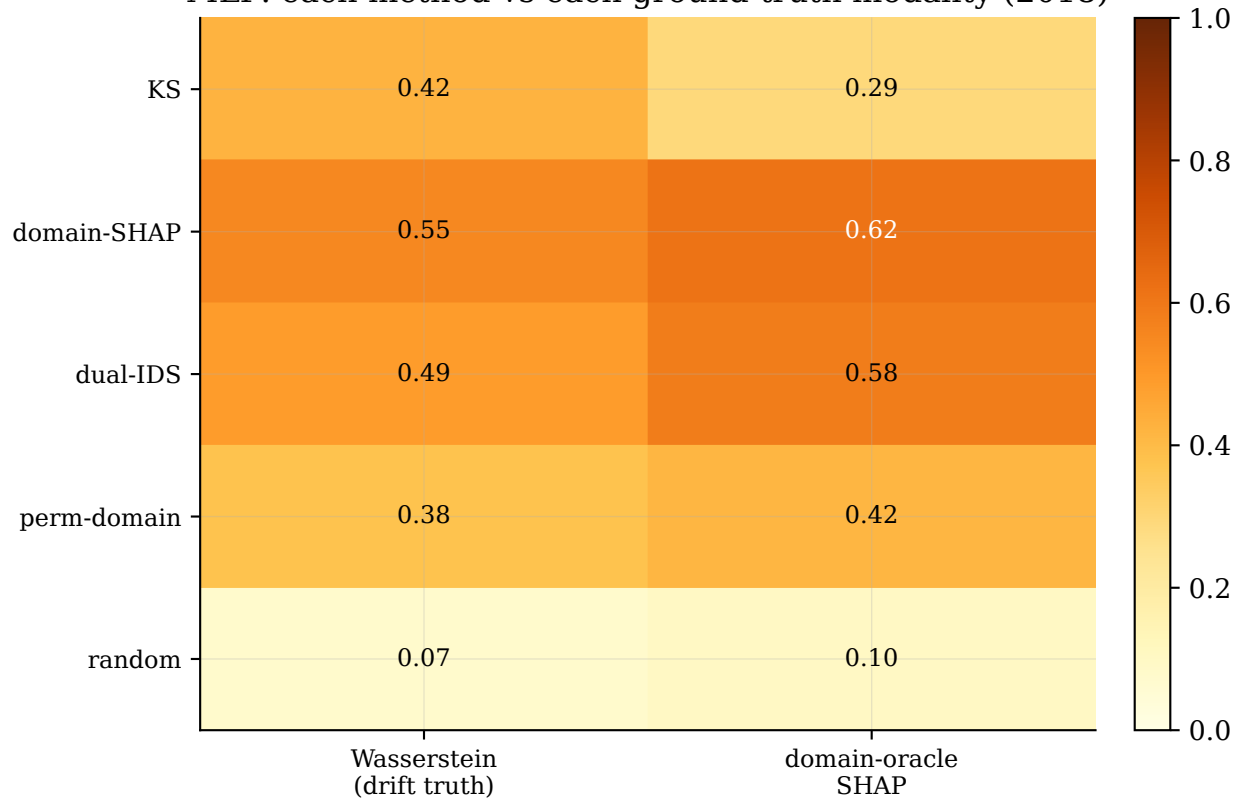
MLP: each method vs each ground-truth modality (2018)
