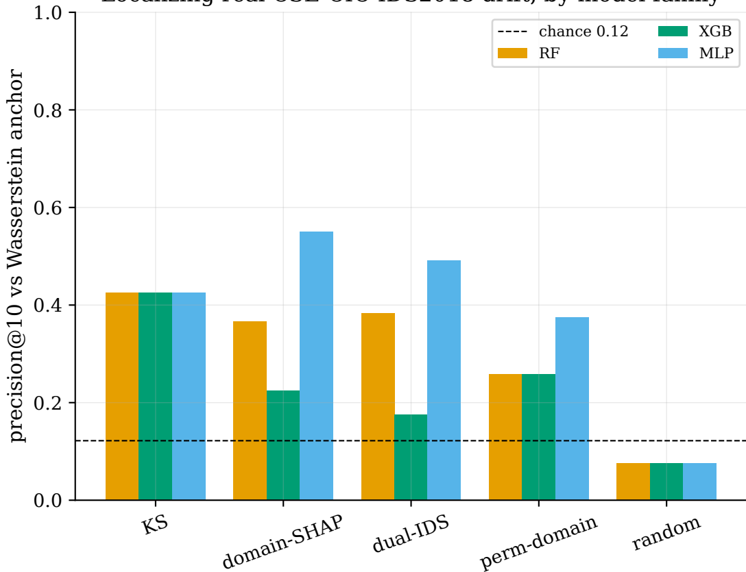
Localizing real CSE-CIC-IDS2018 drift, by model family
